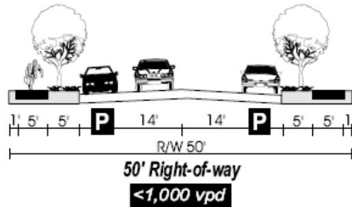
Figure 8-5. Sample Cross Sections for Residential/Local Streets
