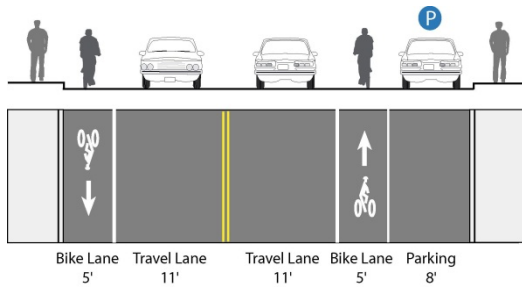
Figure 6-1. Pacific Avenue west of B Street (Existing Conditions)
