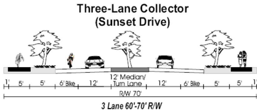
Figure 8-3. Sample Street Cross Sections for Collectors
