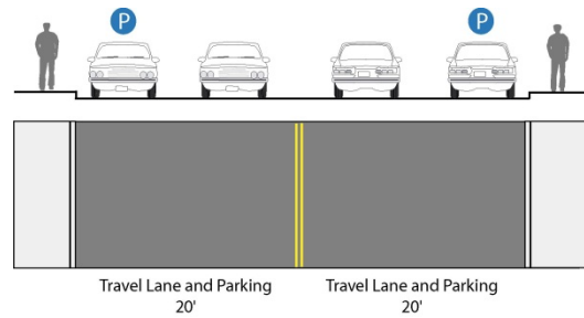
Figure 6-2. Pacific Avenue west of B Street (With Bike Lanes)
