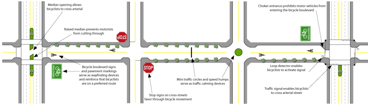
Figure 6-6. Sample Bicycle Boulevard Treatments on a Hypothetical Street
