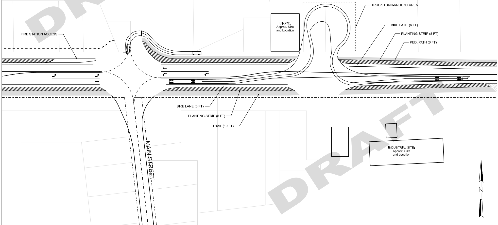
Figure 12. North Access Circulation Concept #2
