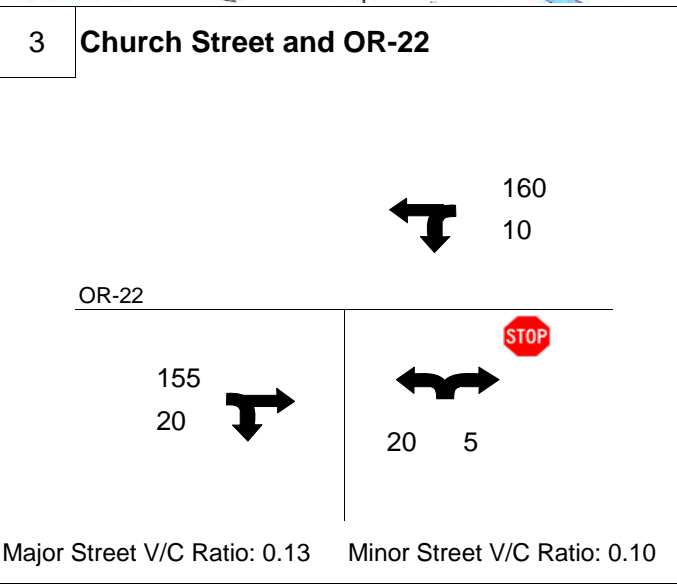
Figure 3 Existing (2005) PM Peak Traffic Operations Idanha Transportation Study
