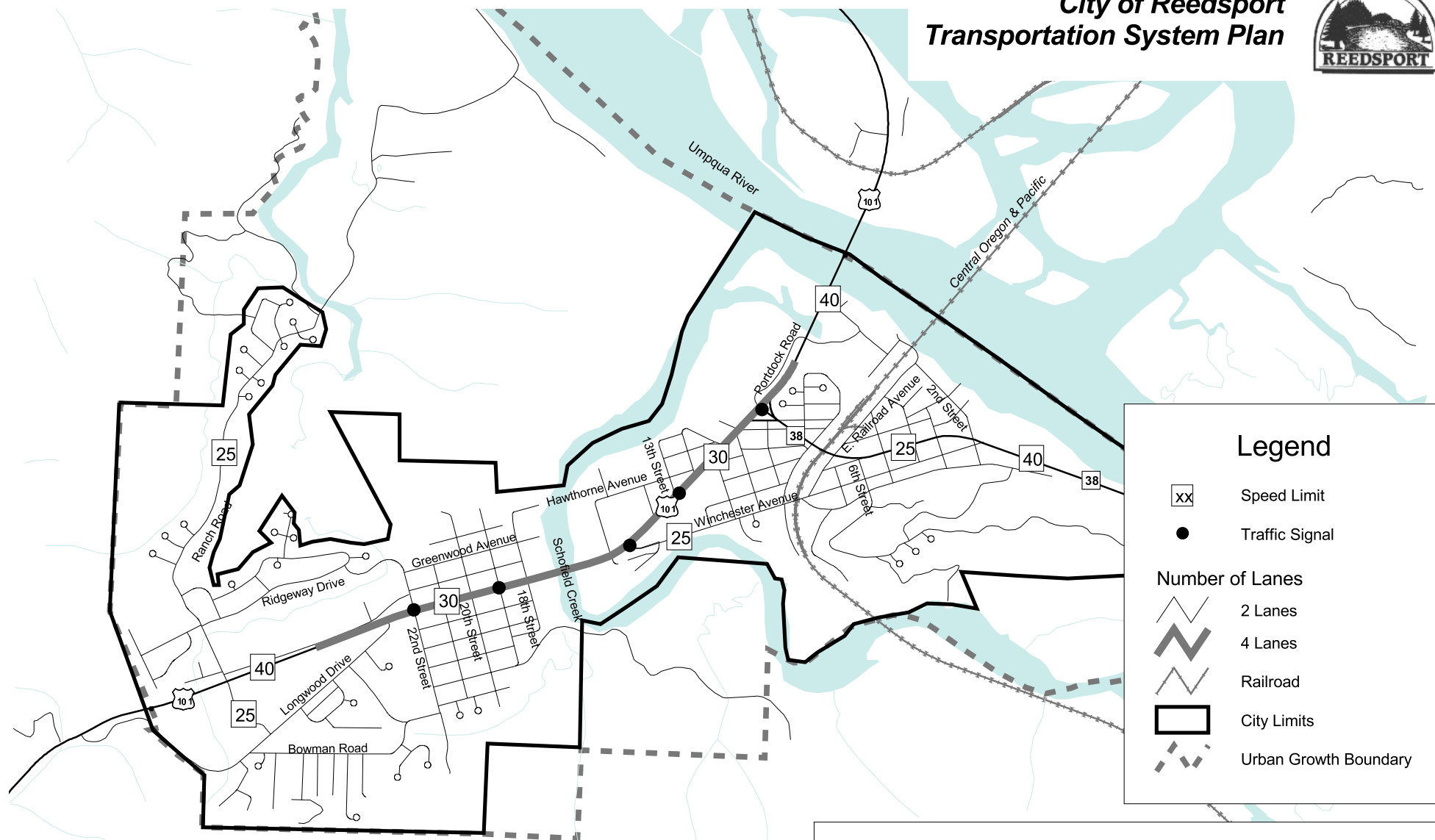
Figure 3-7 ROADWAY CHARACTERISTICS
