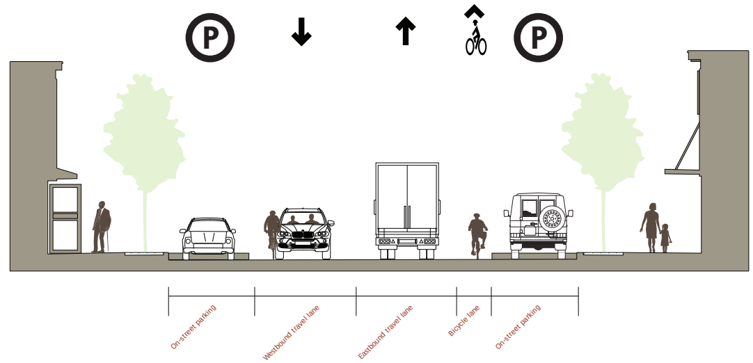
Proposed two-way traffic circulation
