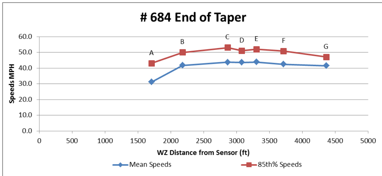
Figure 4.16: Average and 85 th Percentile Speeds of Vehicles for Each Time Segment and Relative Distance from Speed Sensor #684 (End of Taper)
