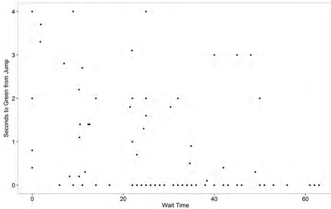
Figure 5-37 Severity of Signal Jump vs. Wait Time
