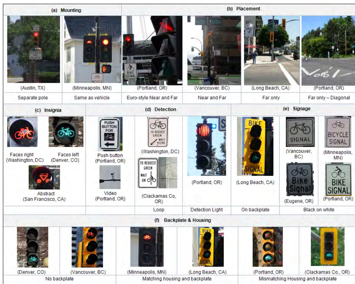
Figure A0-3 Photographs of Various Elements of Bicycle-Specific Traffic Signals
