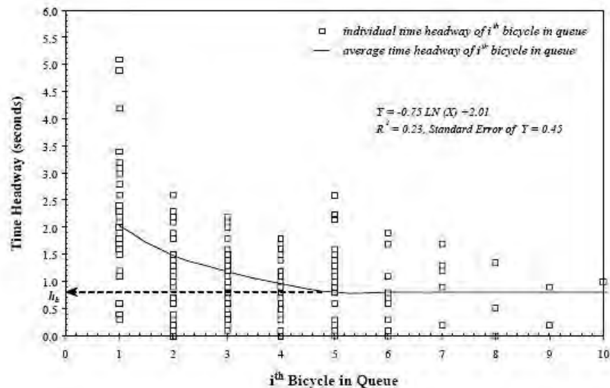
Figure 2-1 Headways of i^{\text{th}} Bicycle in Queue (Raksuntorn and Khan 2003)
