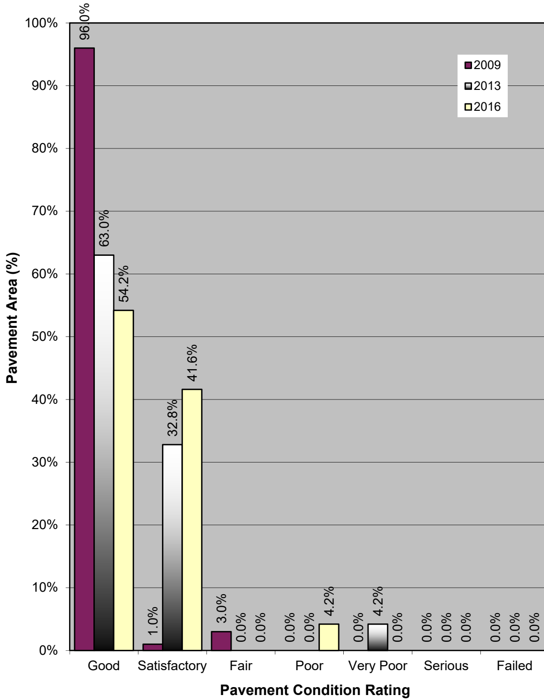
Figure BN-4. Pavement Condition Distribution Bandon State Airport
