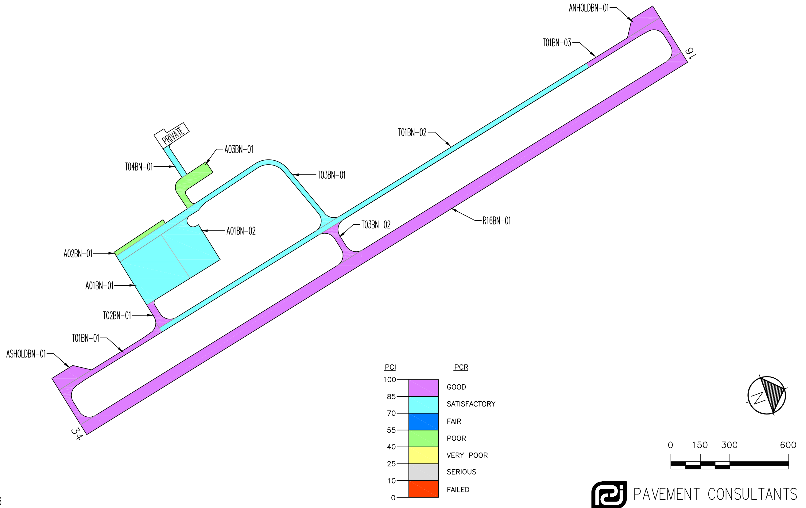
Figure BN-3. Pavement Condition in July 2016. Bandon State Airport
