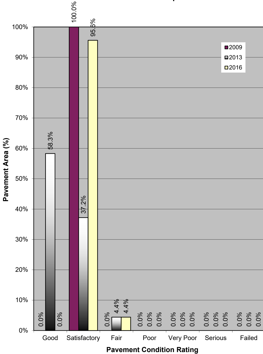
Figure PI-4. Pavement Condition Distribution Pinehurst State Airport
