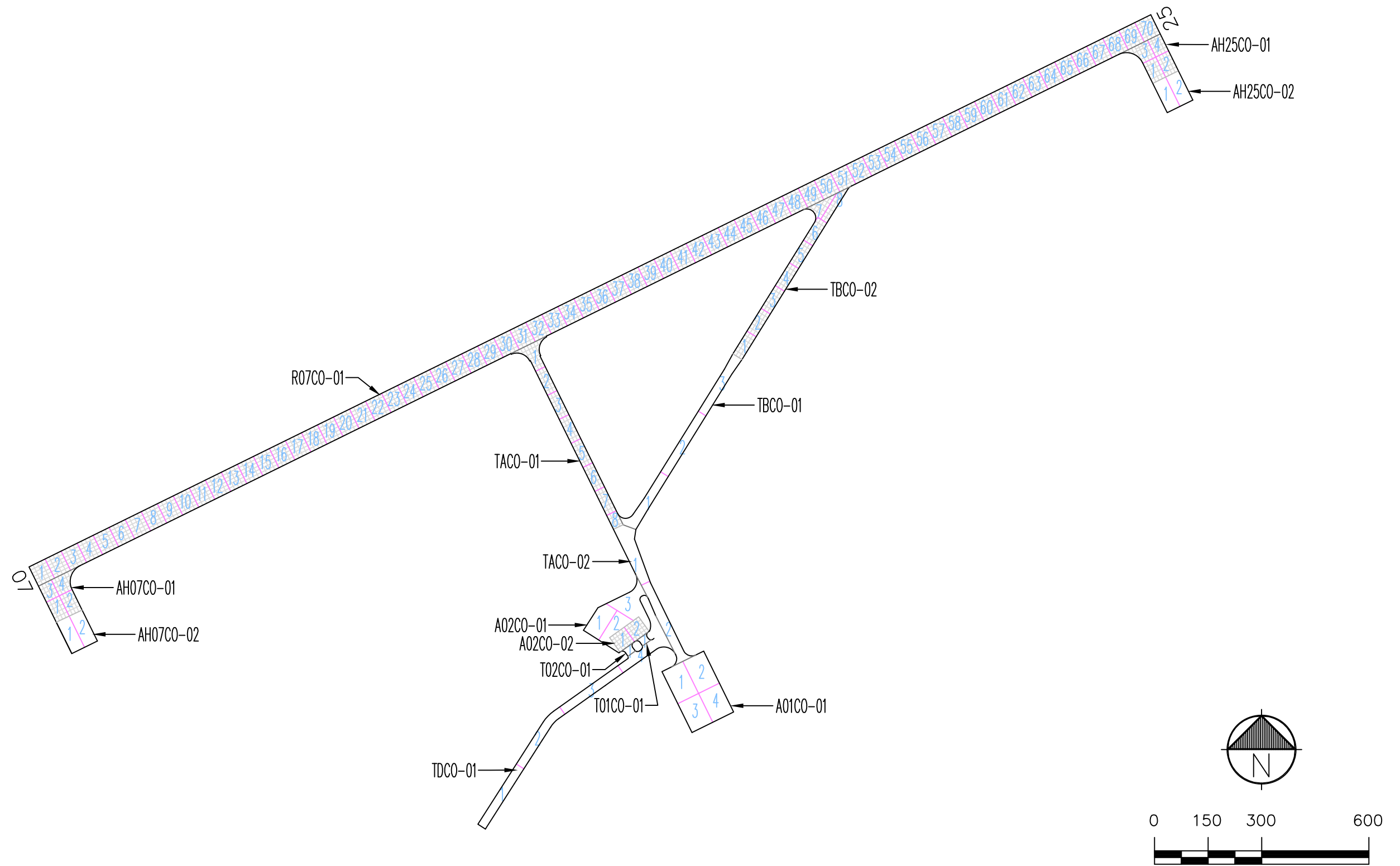
Figure CO-2. Pavement Branch, Section and Sample Unit Layout. Condon State Airport – Pauling Field
