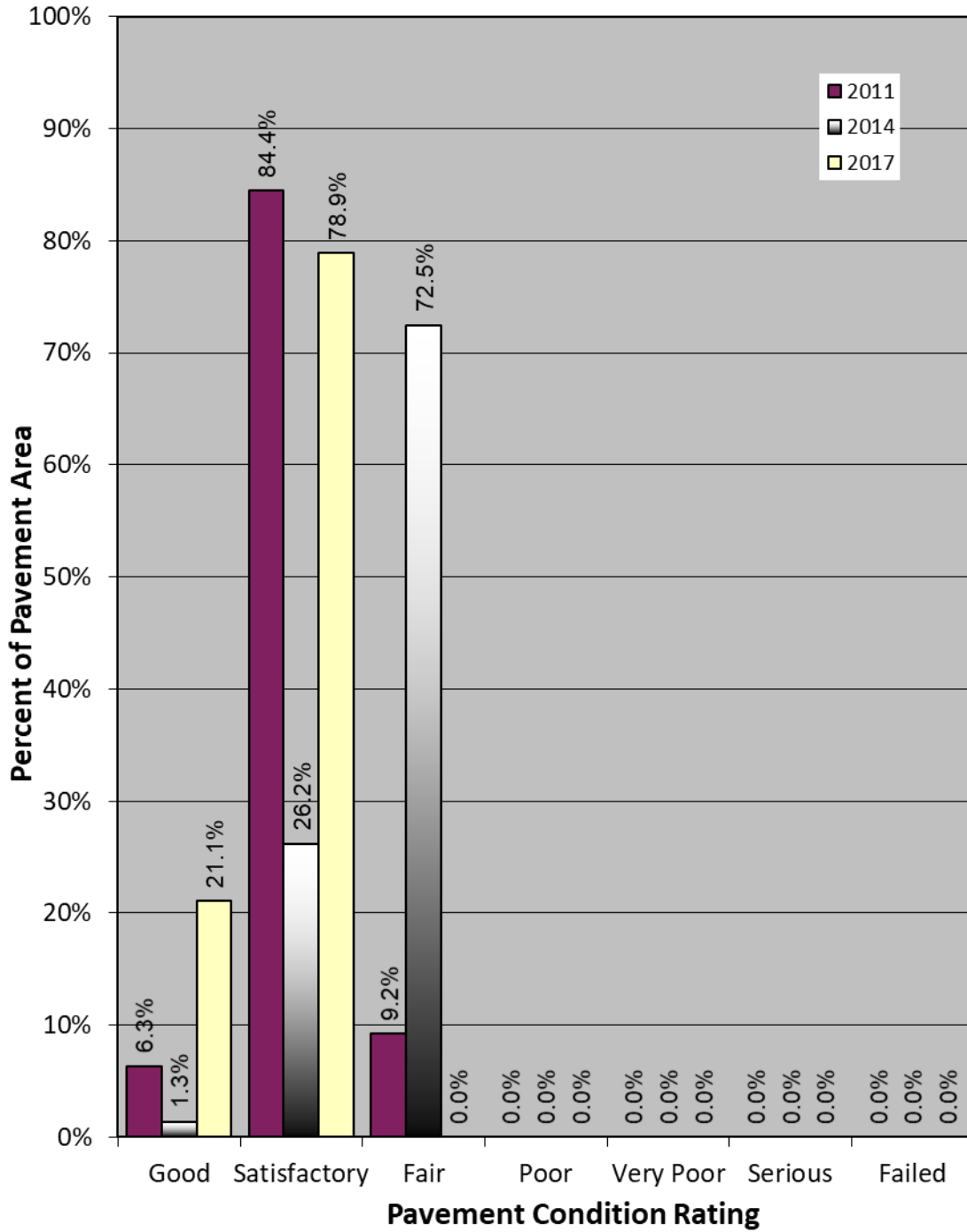
Figure CO-4. Distribution of Pavement Condition Condon State Airport - Pauling Field
