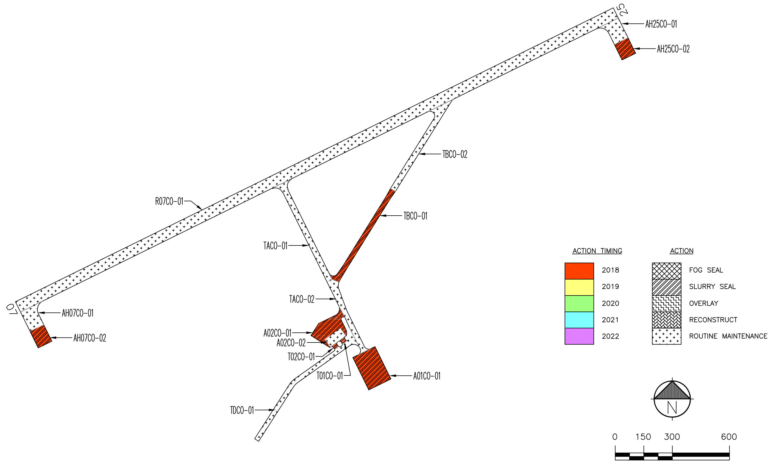
Figure CO-6. Five-Year Pavement Management Plan. Condon State Airport
