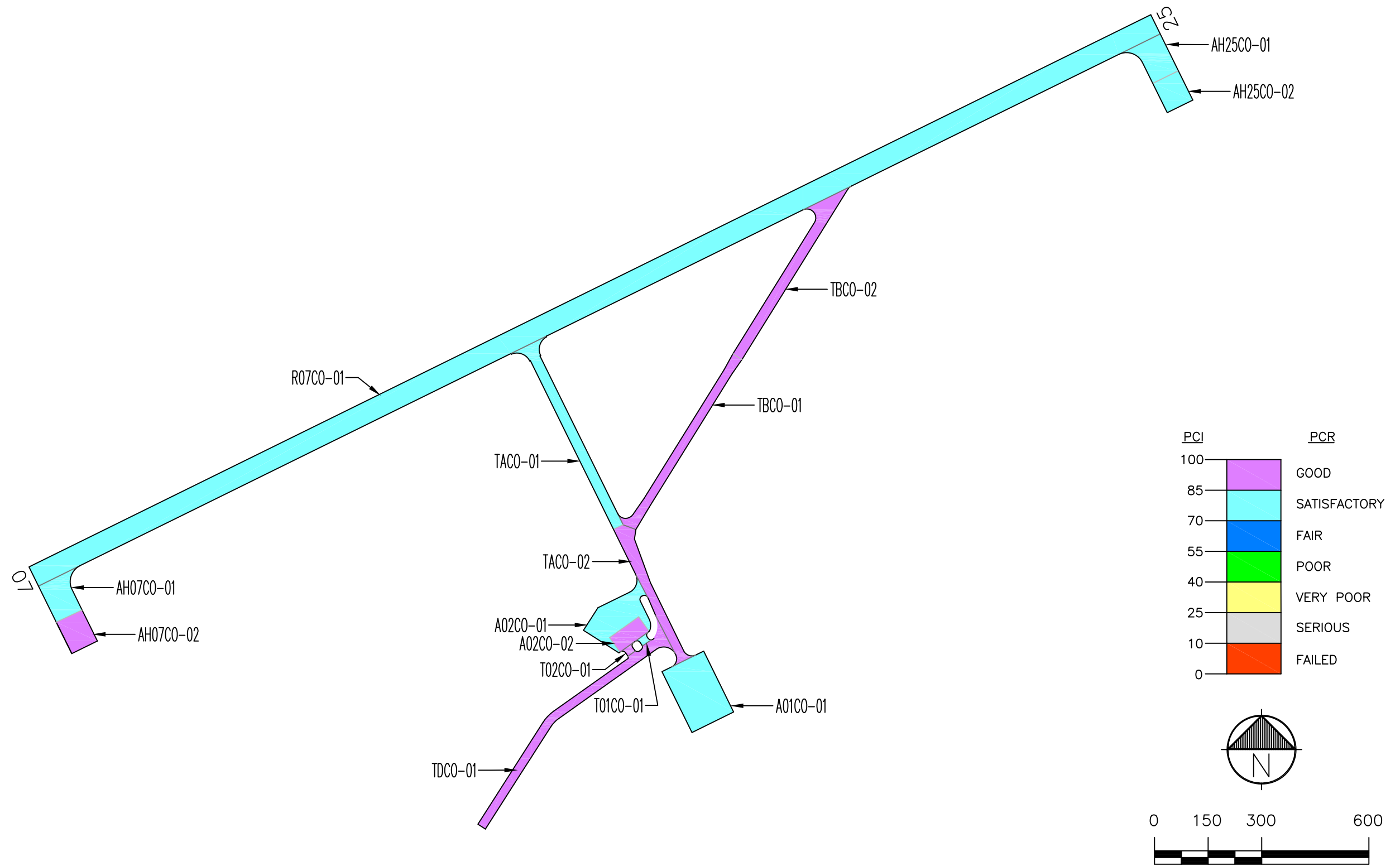
Figure CO-3. Pavement Condition in June 2017. Condon State Airport – Pauling Field
