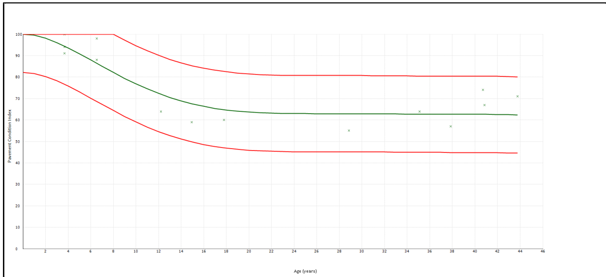
Figure 3. Performance Curve for Category 5 AC Aprons – Eastern Oregon.
