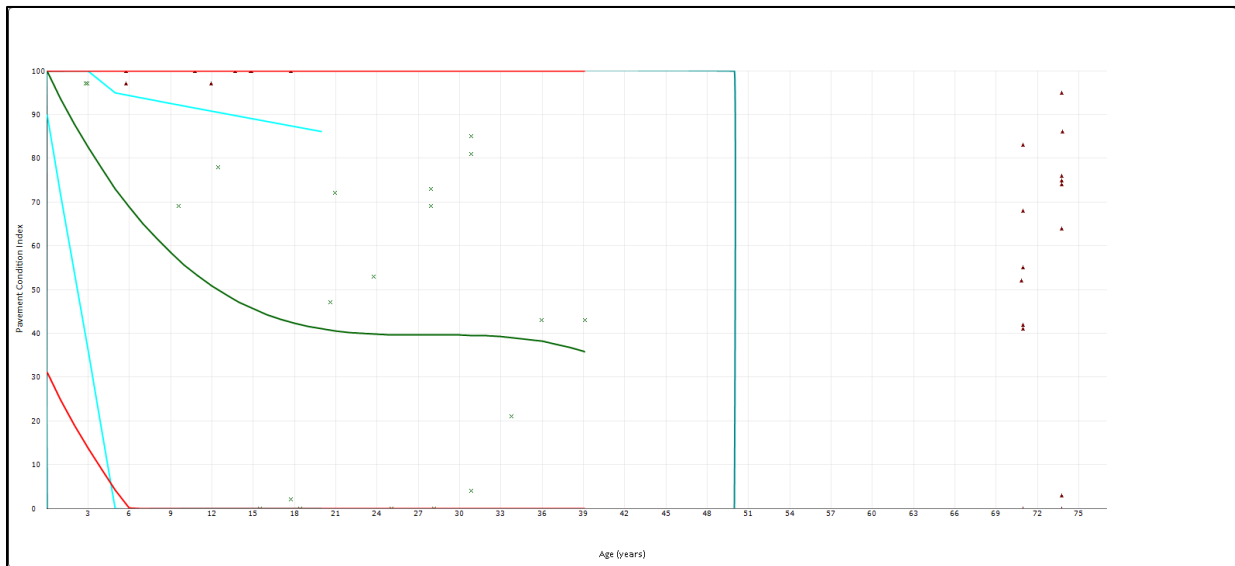
Figure 6. Performance Curve for Category 5 PCC Aprons – Eastern Oregon.
