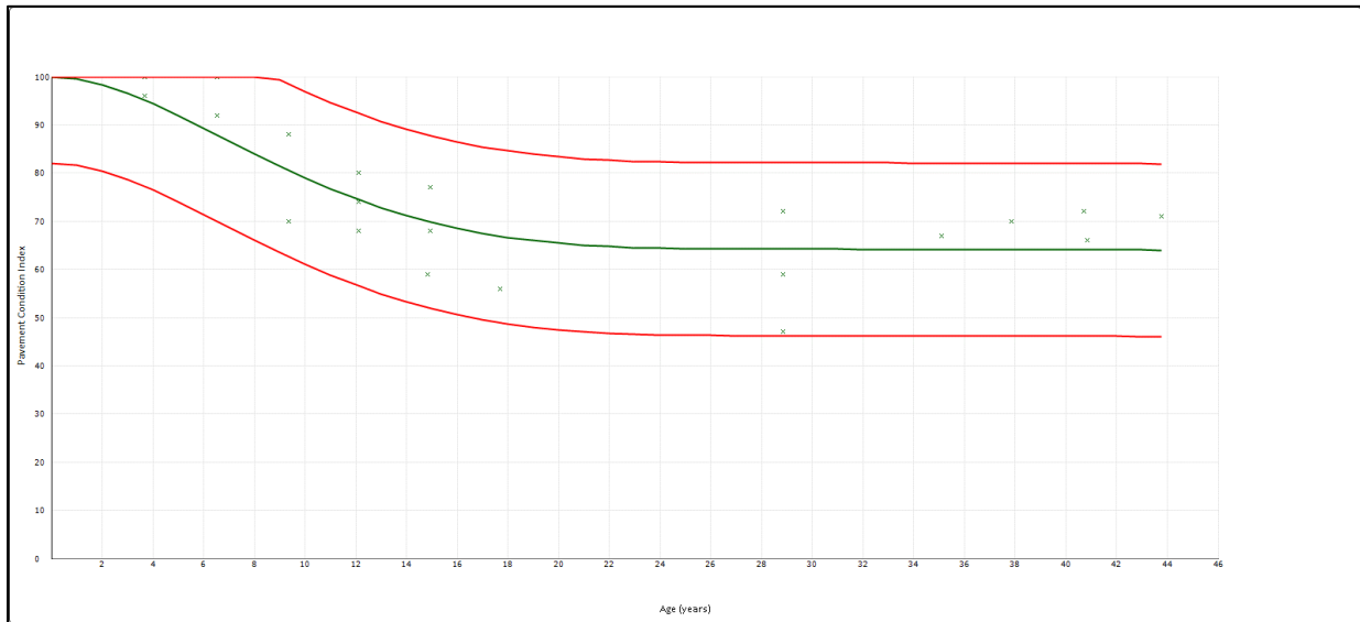
Figure 5. Performance Curve for Category 5 AC Taxiways – Eastern Oregon.
