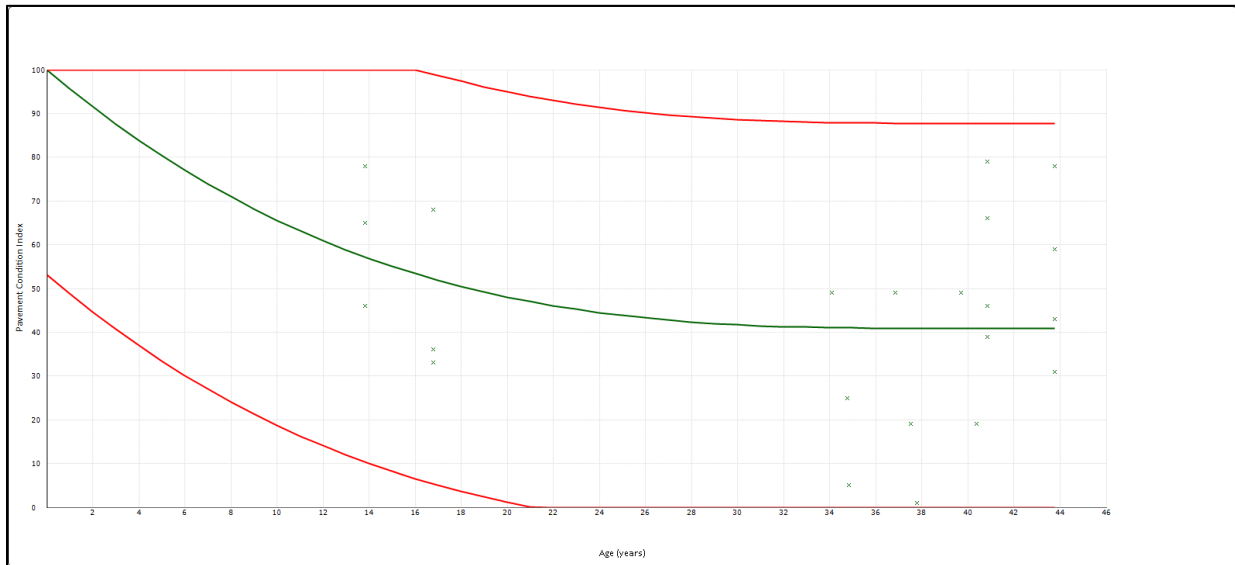
Figure 9. Performance Curve for Category 5 ST Runways – Eastern Oregon.
