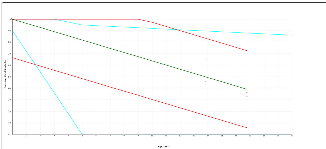
Figure 10. Performance Curve for Category 5 ST Taxiways – Eastern Oregon.
