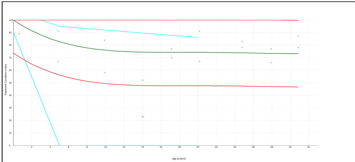
Figure 7. Performance Curve for Category 5 PCC Taxiways – Eastern Oregon.
