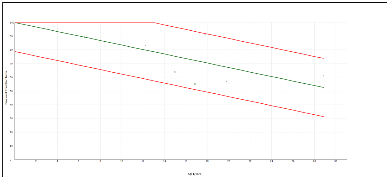
Figure 4. Performance Curve for Category 5 AC Runways – Eastern Oregon.
