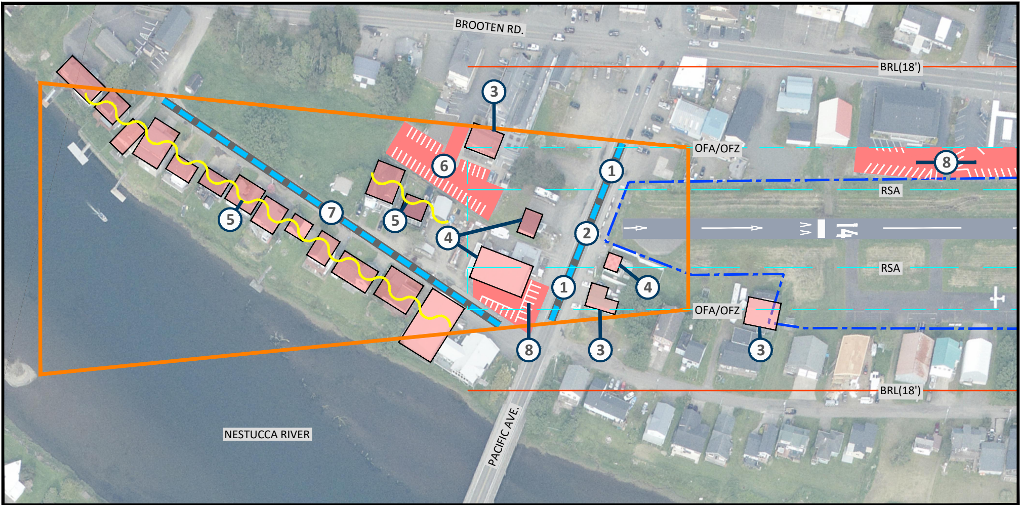
DETAIL A SCALE: 1"=150'
