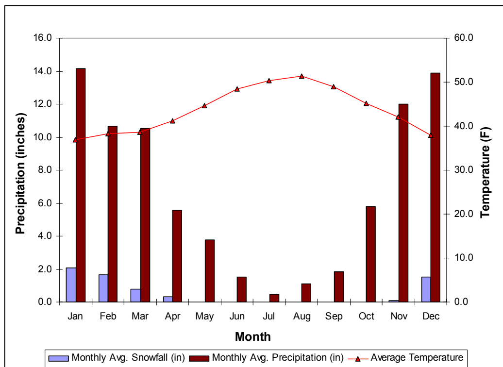
Figure 2-4. Climagraph for CA4577 (Klamath River Mouth).
