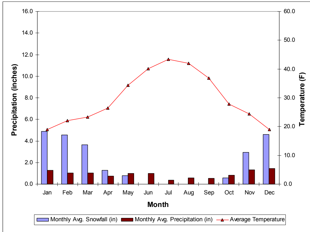
Figure 2-3. Climagraph for CA9053 (Tule Lake).
