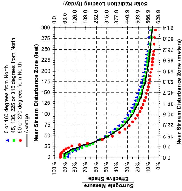
Figure 3-18. Shade Curves – Deciduous Potential Land Cover
