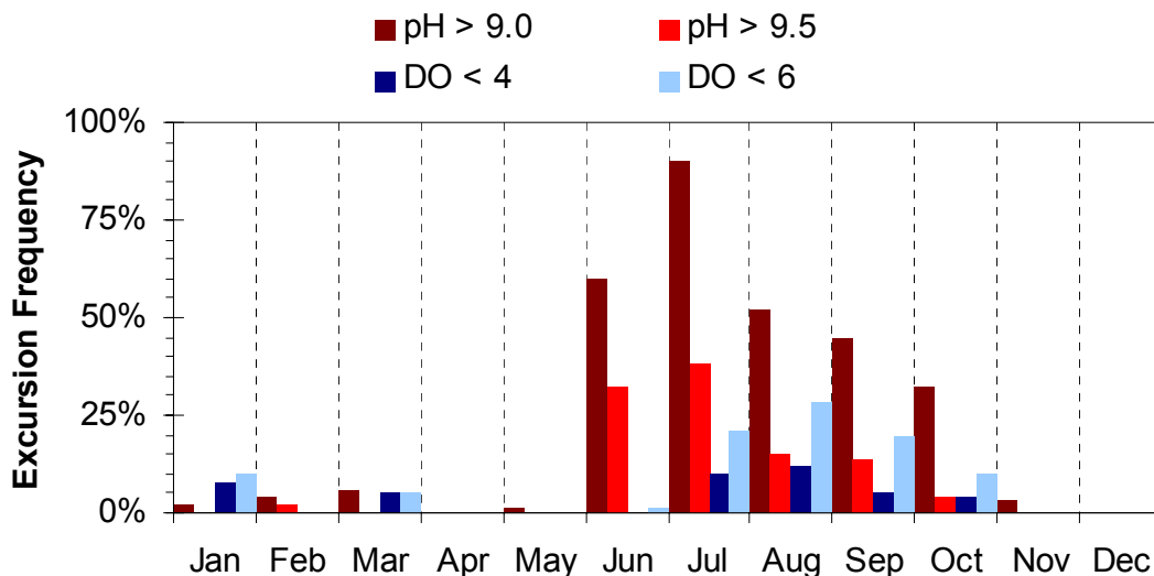
Figure 2-4. Seasonal Excursions Frequencies above Water Quality Standards
