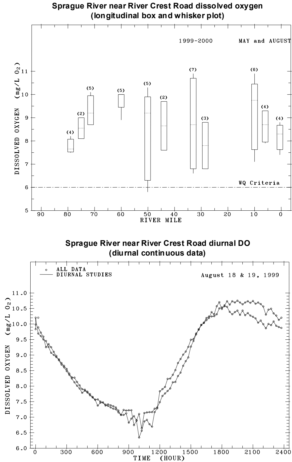
Figure 4-2. Sprague River near River Crest Road dissolved oxygen
