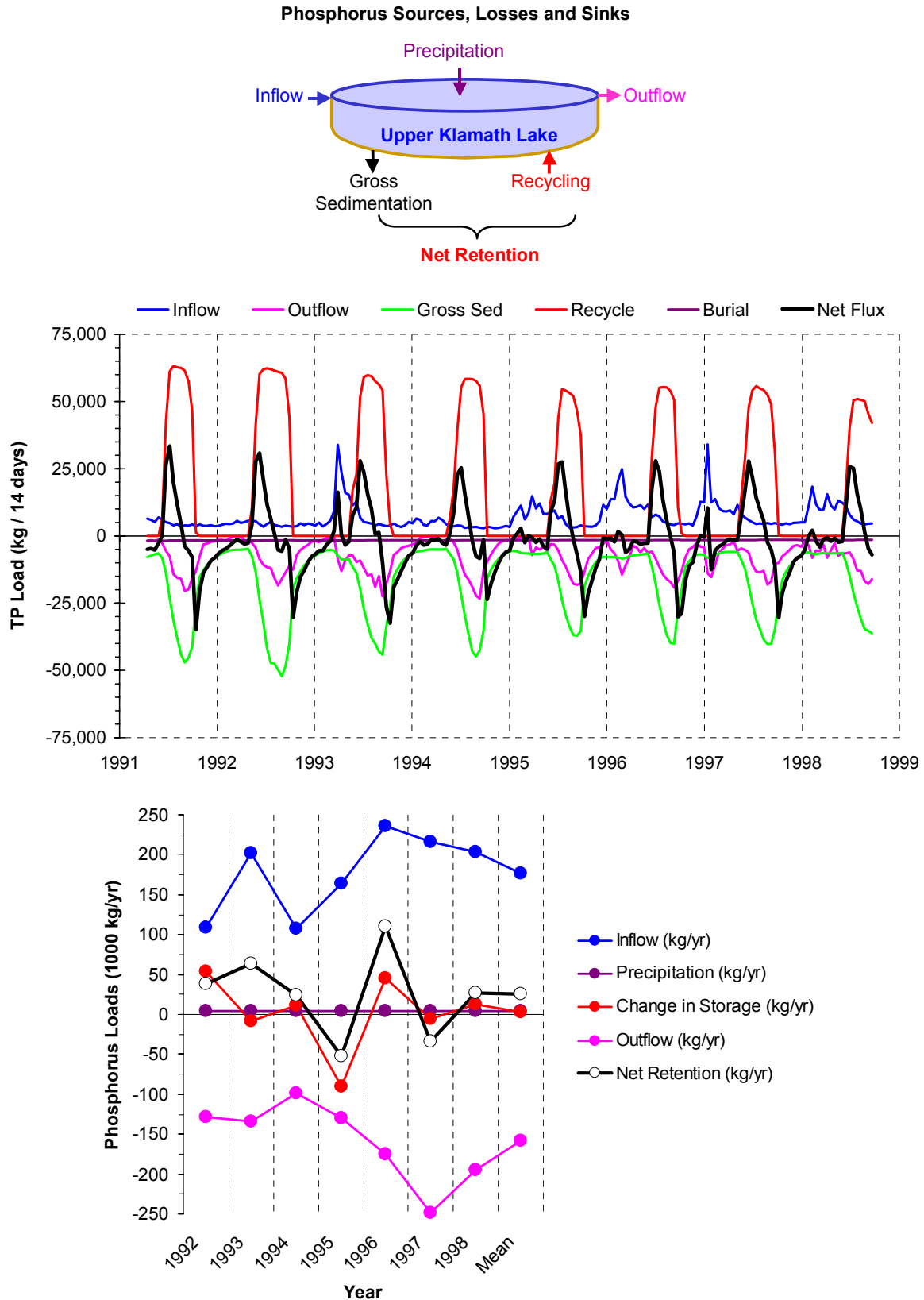
Figure 2-21. Time Series Total Phosphorus Flux Mass Balance Pathways - Inflow, Outflow, Gross Sedimentation and Recycling (Walker, 2001)
