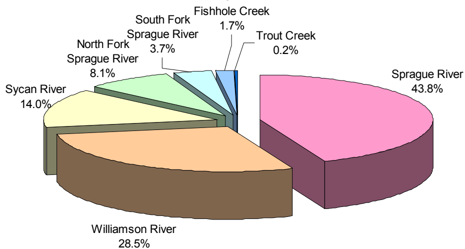
Distribution of the Total Nonpoint Source Solar Heat Load
