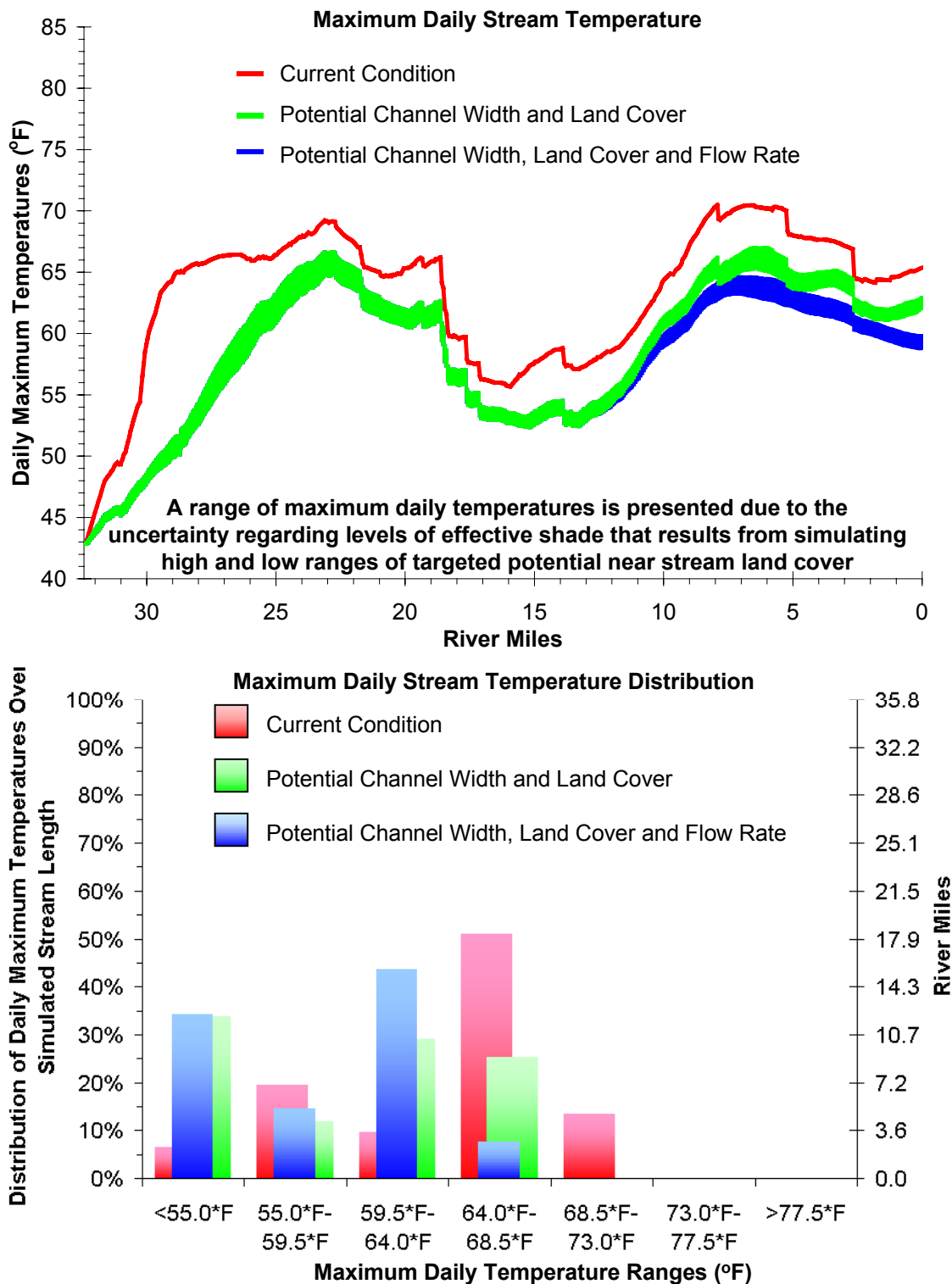
Figure 3-23. North Fork Sprague River Daily Maximum Temperature Distribution (Current Condition and Allocated Condition) (August 16, 1999)
