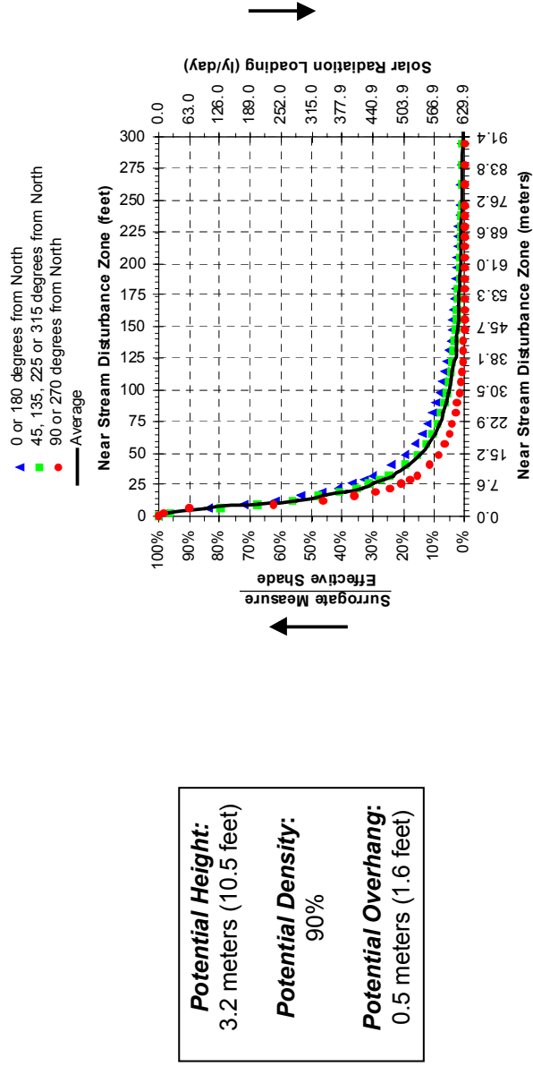
Figure 3-20. Shade Curve – Wetland Shrub Potential Land Cover
