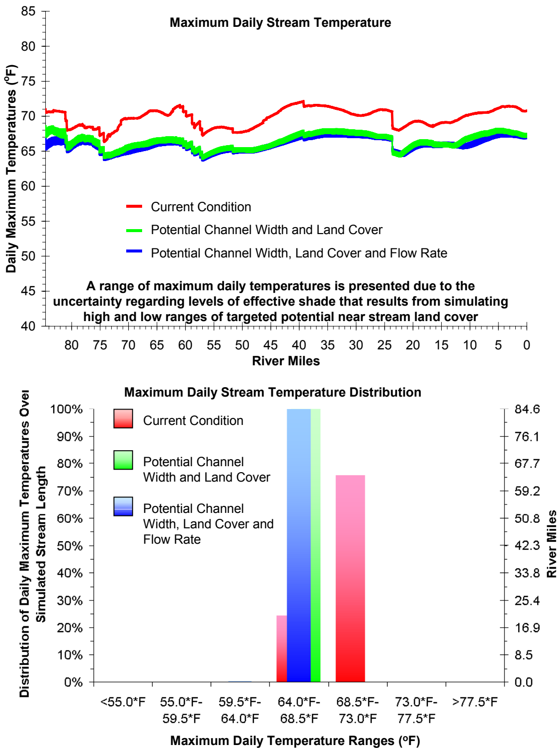
Figure 3-26. Sprague River Daily Maximum Temperature Distribution (Current Condition and Allocated Condition) (August 12, 1999)
