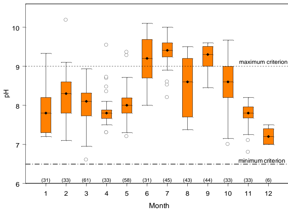
Figure 2-11. Seasonal box plot of pH at Link River.
