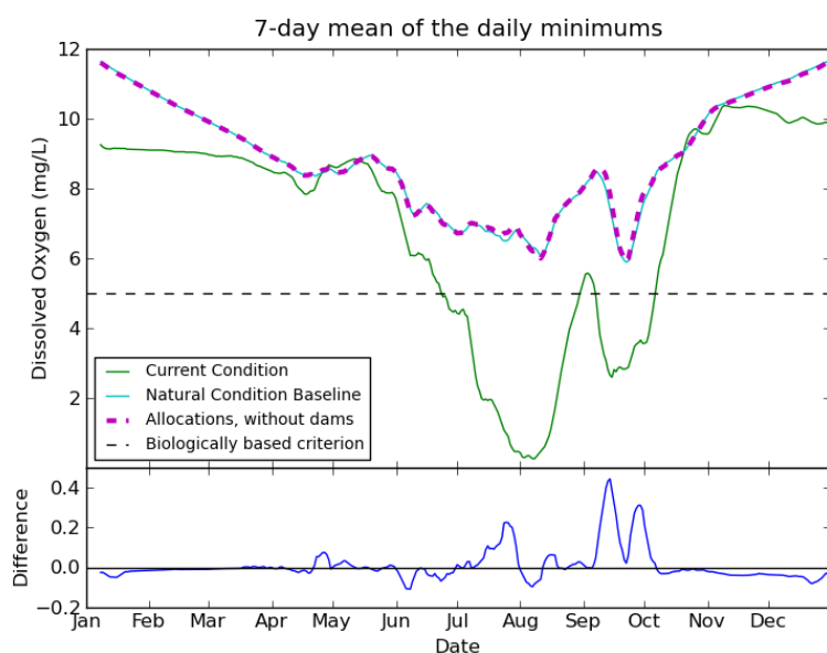
Figure 2-30. Predicted DO (7-day metric) in Klamath River at Klamath Falls WWTP outfall location. The 'Difference' at the bottom of the figure shows the 'Allocations, without dams' minus the 'Natural Condition Baseline Scenario'.
