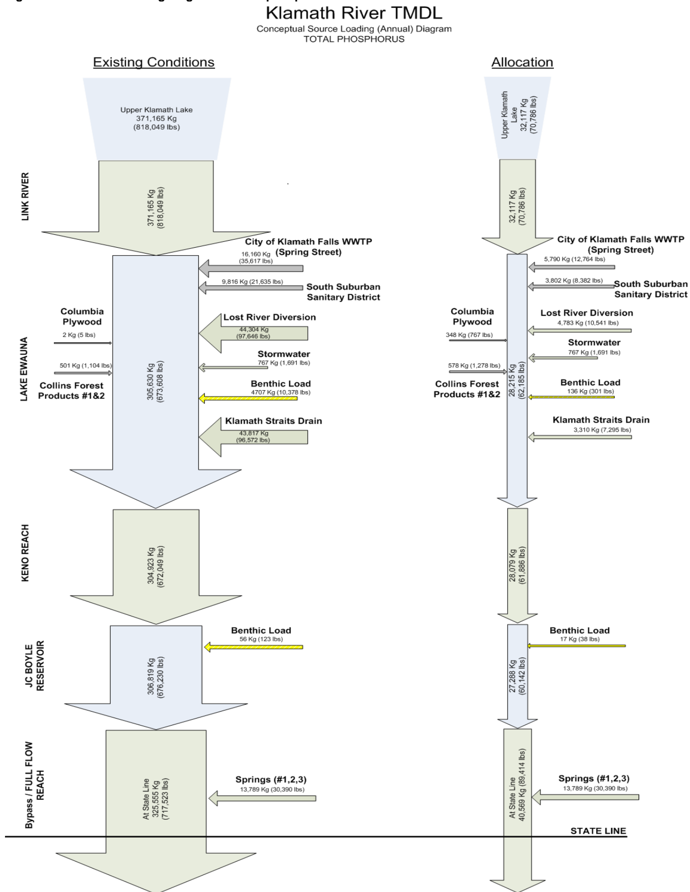
Figure 2-36. Annual loading diagram for total phosphorus
