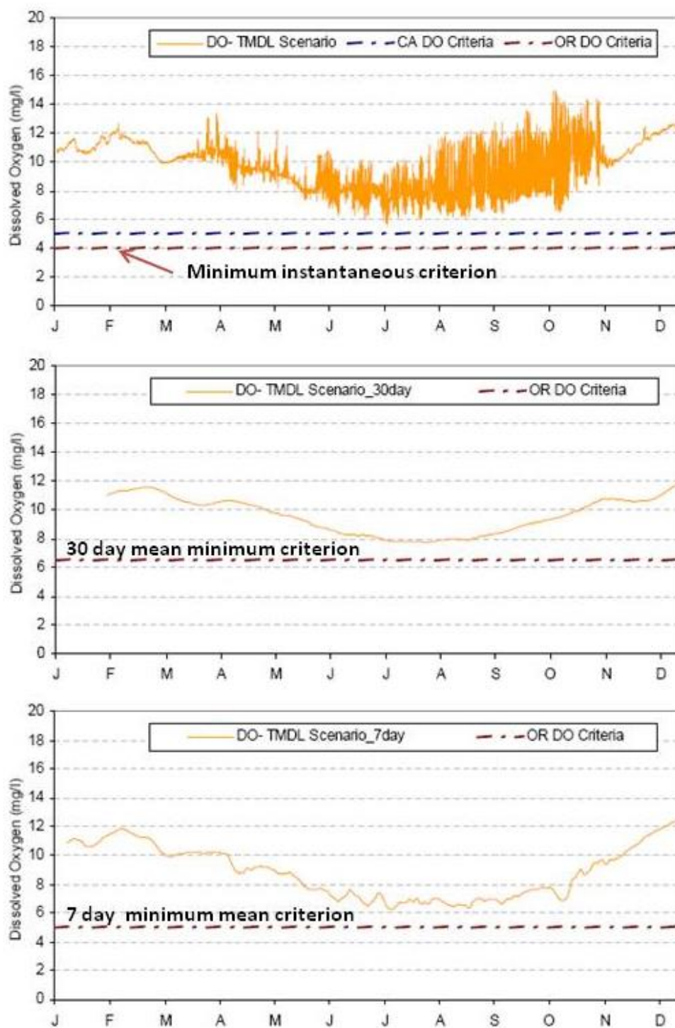
Figure 3-21. DO standard compliance – Stateline Road (LRSR).
