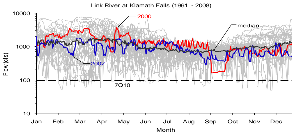
Figure 2-13. Flow measurements at Link River. The hydrographs of every year except those being modeled are in gray.
