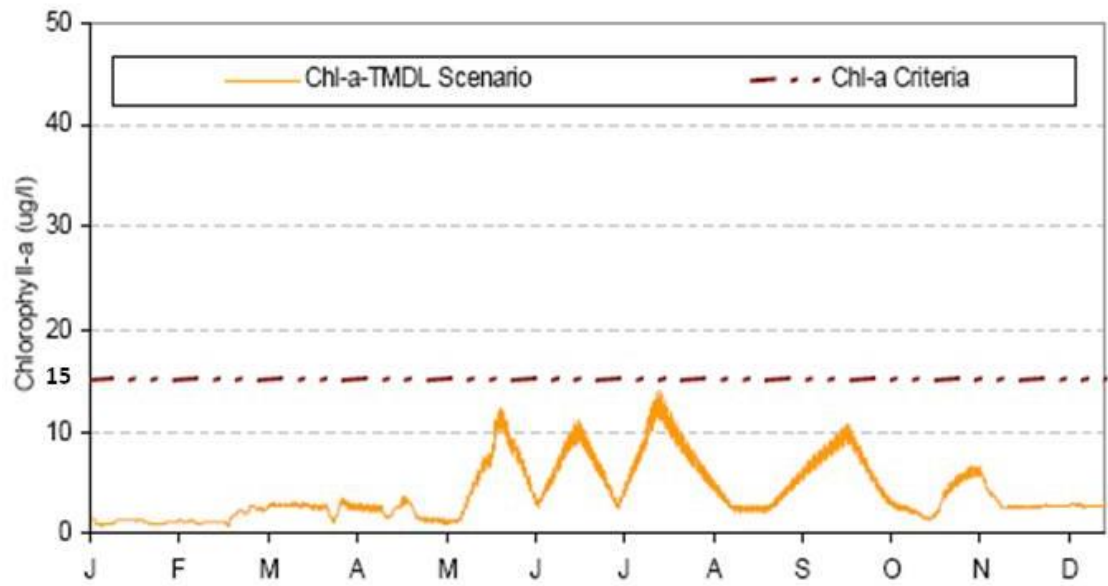
Figure 3-19. Chlorophyll-a standard (15µg/l) compliance – Harpold Dam (LRHD).
