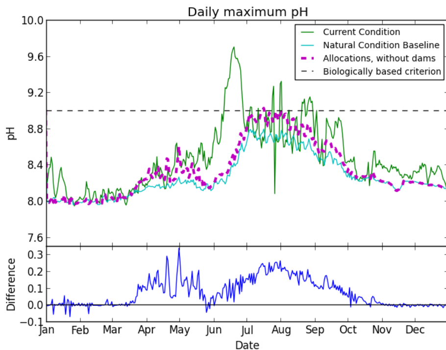
Figure 2-35. Predicted daily maximum pH in Klamath River at stateline. The 'Difference' at the bottom of the figure shows the 'Allocations, without dams' minus the 'Natural Condition Baseline Scenario'.
