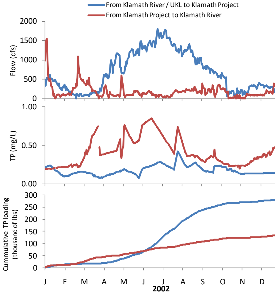
Figure 2-18. Flow, concentration and cumulative loading analysis of USBR's Klamath Project. Total phosphorus (TP) concentrations weighted based on relative flow rates.
