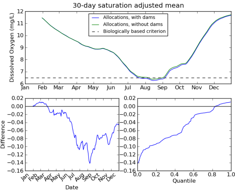
Figure 2-40. Predicted DO (30-day metric) in Klamath River at the deepest point in JC Boyle Reservoir, depth averaged. The 'Difference' at the bottom-left of the figure shows the 'Allocations, with dams' scenario minus the 'Allocations, without dams' scenario. The 'Quantile' plot at the bottom-right shows the distribution of the differences.
