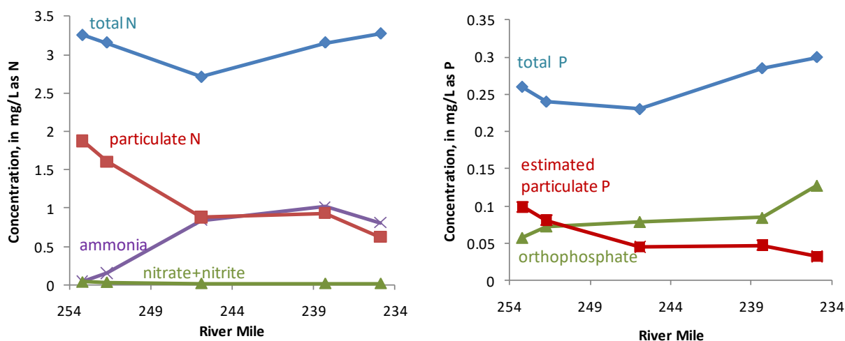
Figure 2-21. Nitrogen (N) and phosphorus (P) compounds in Keno impoundment, upstream is to the left, at the mouth of Link River. Data from Sullivan et al. (2009), median 7/15/2008 to 9/15/2008 concentrations.
