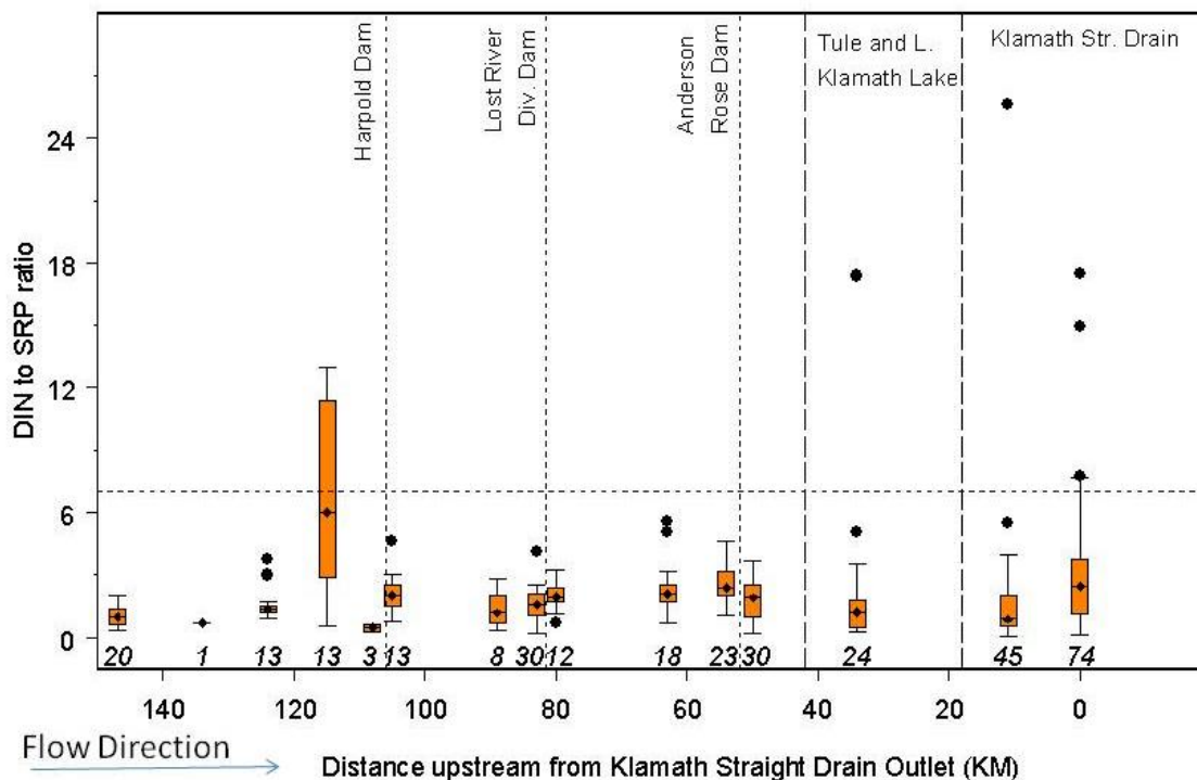
Figure 3-10. Longitudinal plot of the ratio of dissolved inorganic nitrogen (DIN) to soluble reactive phosphorus (SRP), July through September. A ratio of 7 where points above this line indicate possible phosphorus limitation and points below this line indicate possible nitrogen limitation.
