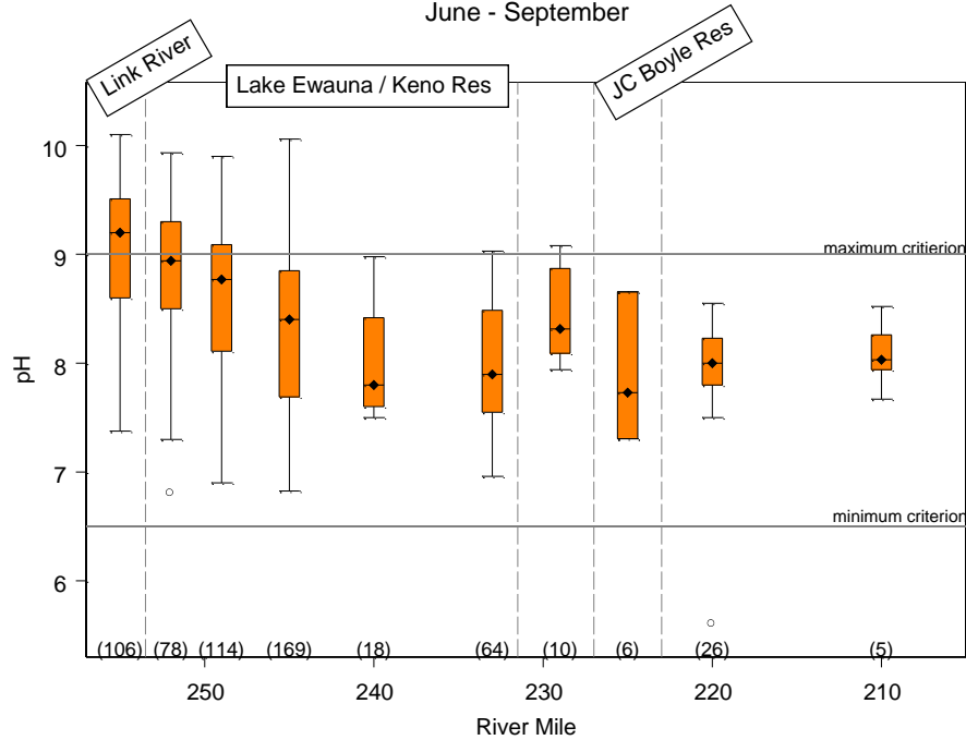
Figure 2-6. pH longitudinal profile of the Klamath River from the Oregon / California border to Upper Klamath Lake. June - September
