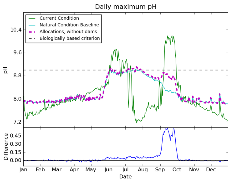
Figure 2-34. Predicted pH in Klamath River at South Suburban WWTP outfall location.
