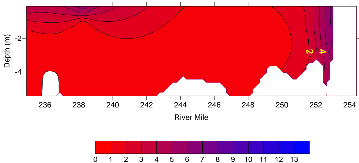
Figure 2-2. Keno impoundment longitudinal cross section of dissolved oxygen (mg/l) on July 26 2005 (Deas 2008).
