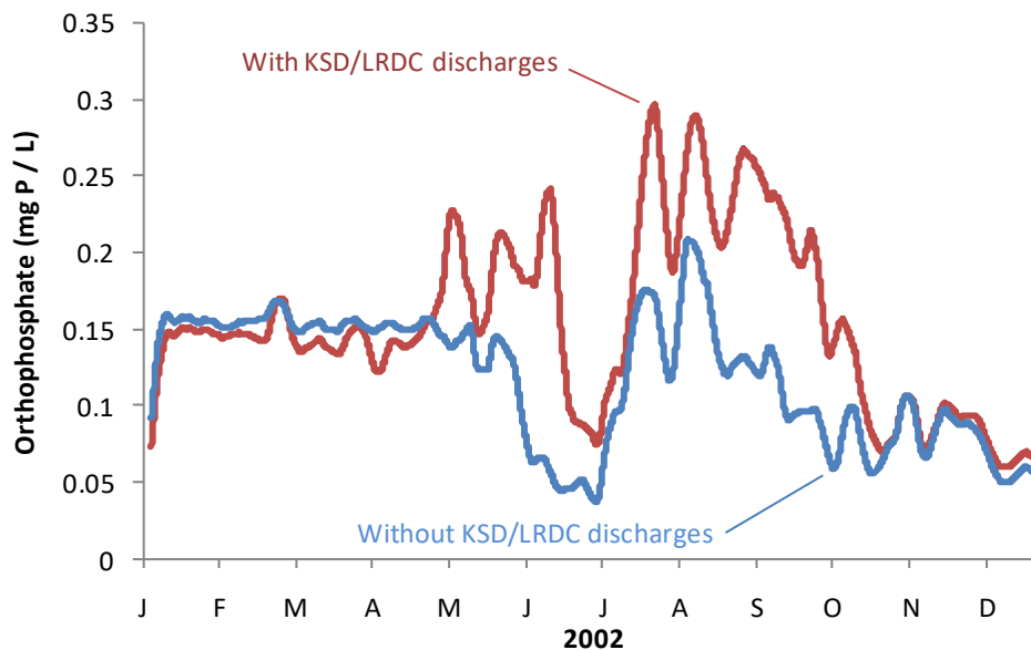
Figure 2-20. Klamath River (Keno impoundment) model results from just downstream of Klamath Straits Drain discharge. The “With KSD/LRDC” results are from the 2002 calibration model. The “Without ...” results are from a scenario exactly like the 2002 calibration except the constituent concentrations of parameters for Lost River Diversion and Klamath Straits Drain were set to the same constituent concentrations as Link River.
