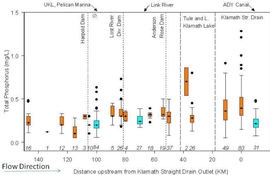
Figure 3-12. Total phosphorus concentrations measured in the Lost River system July through September. The number above the x-axis represents the number of data points used to construct each box plot.
