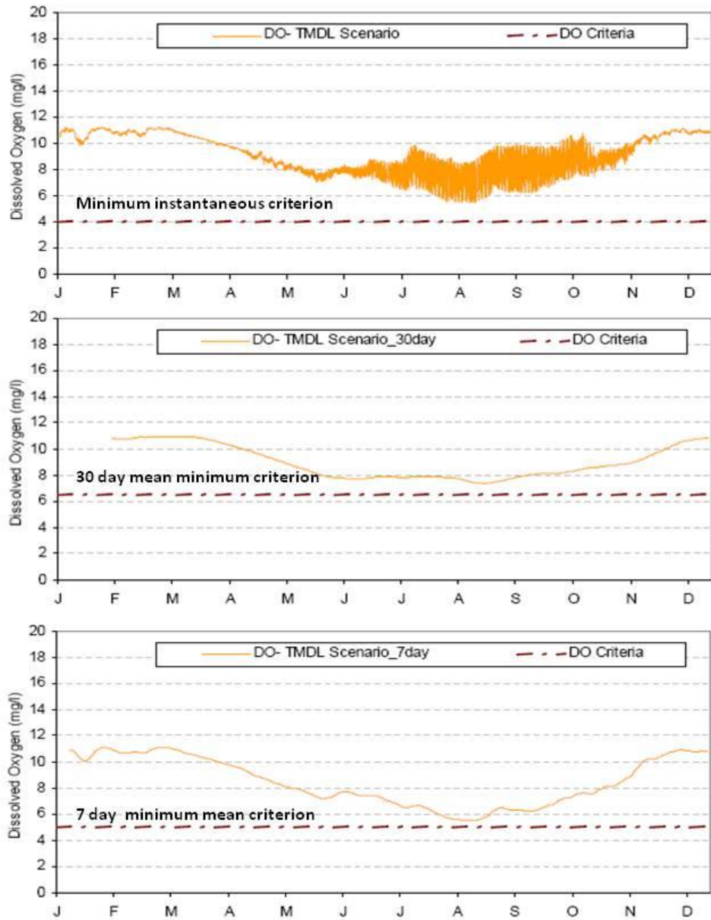
Figure 3-17. Dissolved Oxygen Standards Compliance – Harpold Dam (LRHD).
