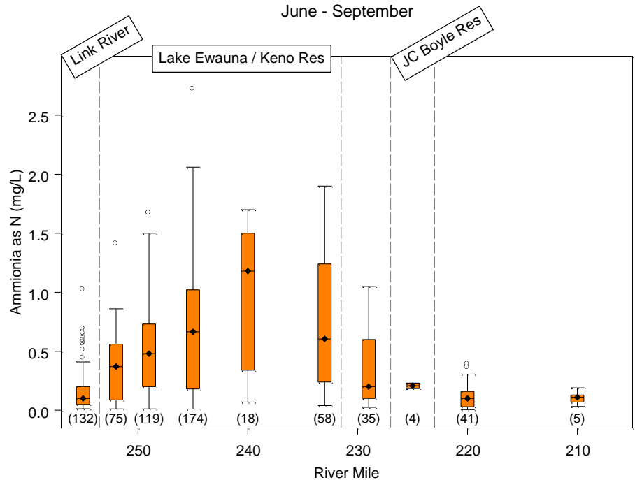
Figure 2-4. Ammonia longitudinal profile of the Klamath River from Upper Klamath Lake to the Oregon / California border. Miller Island is river mile 245.
