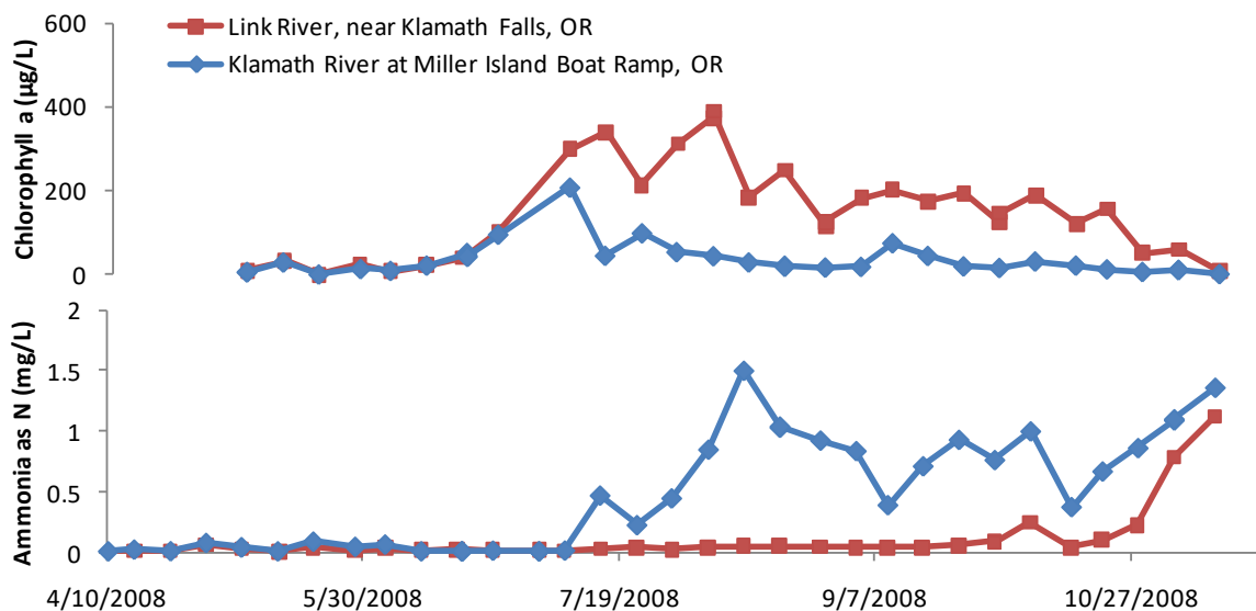
Figure 2-22. Time series of chlorophyll a and ammonia concentrations.
