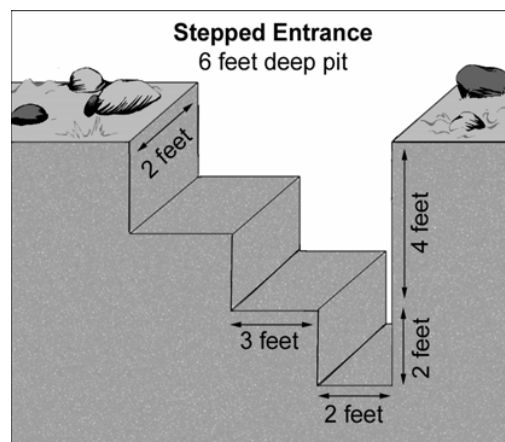
The entrance to a six-foot test pit may be sloped or stepped as soil conditions warrant.
