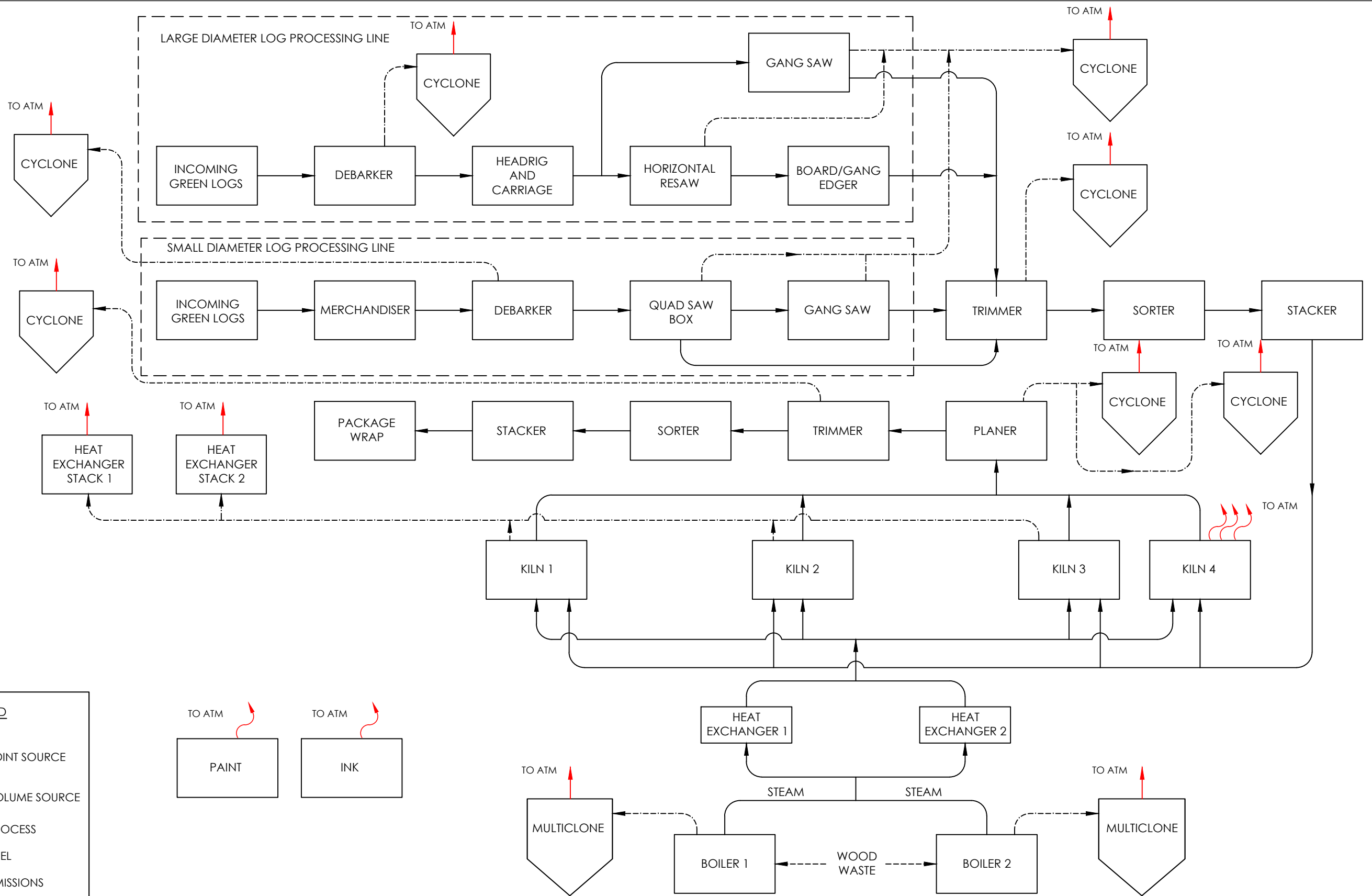
Figure 2-3 Process Flow Diagram Collins Pine Company Lakeview, Oregon
