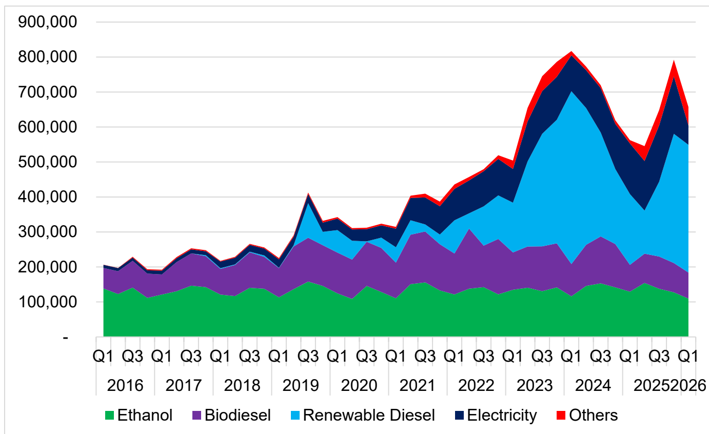
Figure 2. Credits in metric tons CO2e by fuel type, Q1 2016 – Q1 2026
