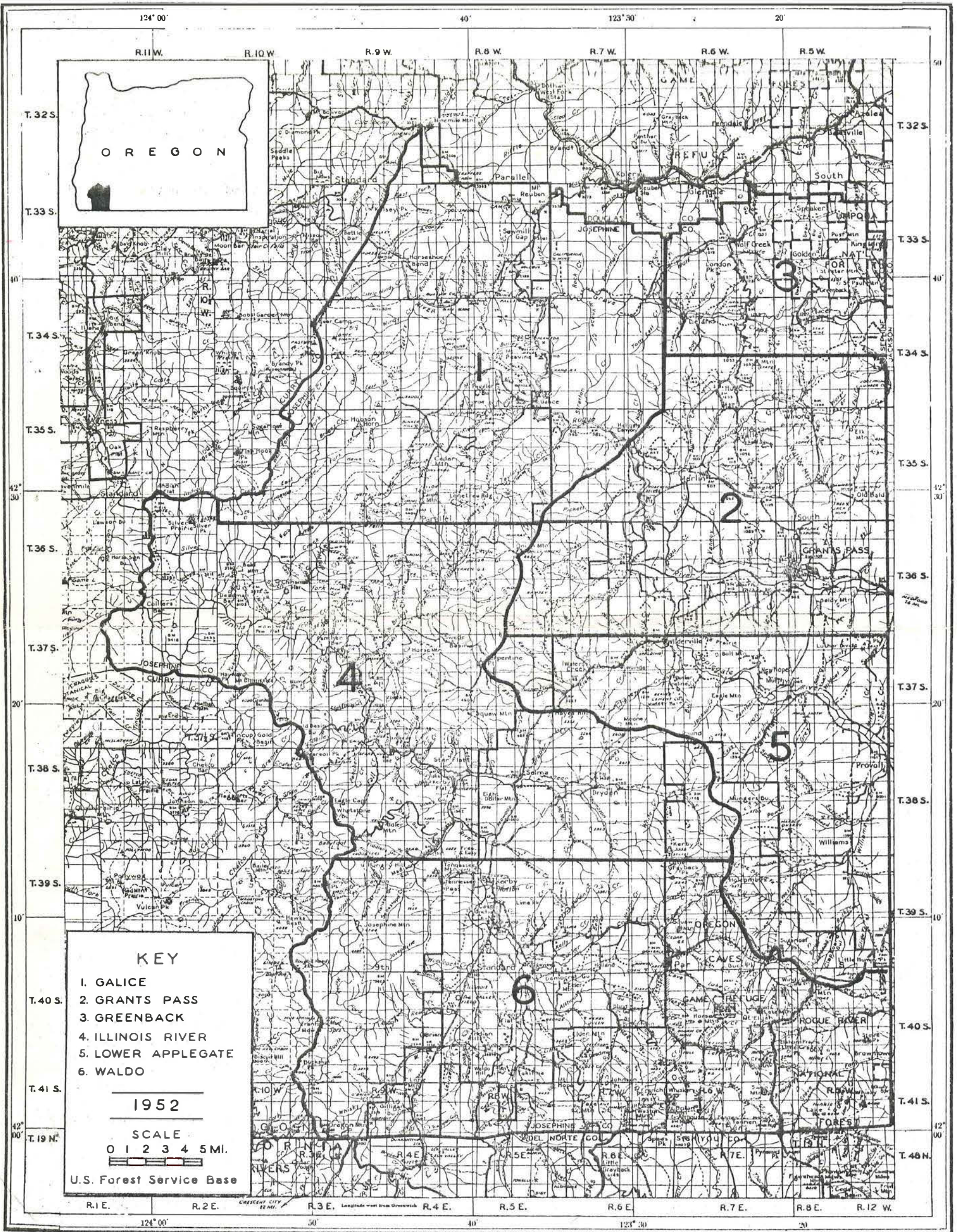
MINING AREAS OF JOSEPHINE COUNTY, OREGON.
