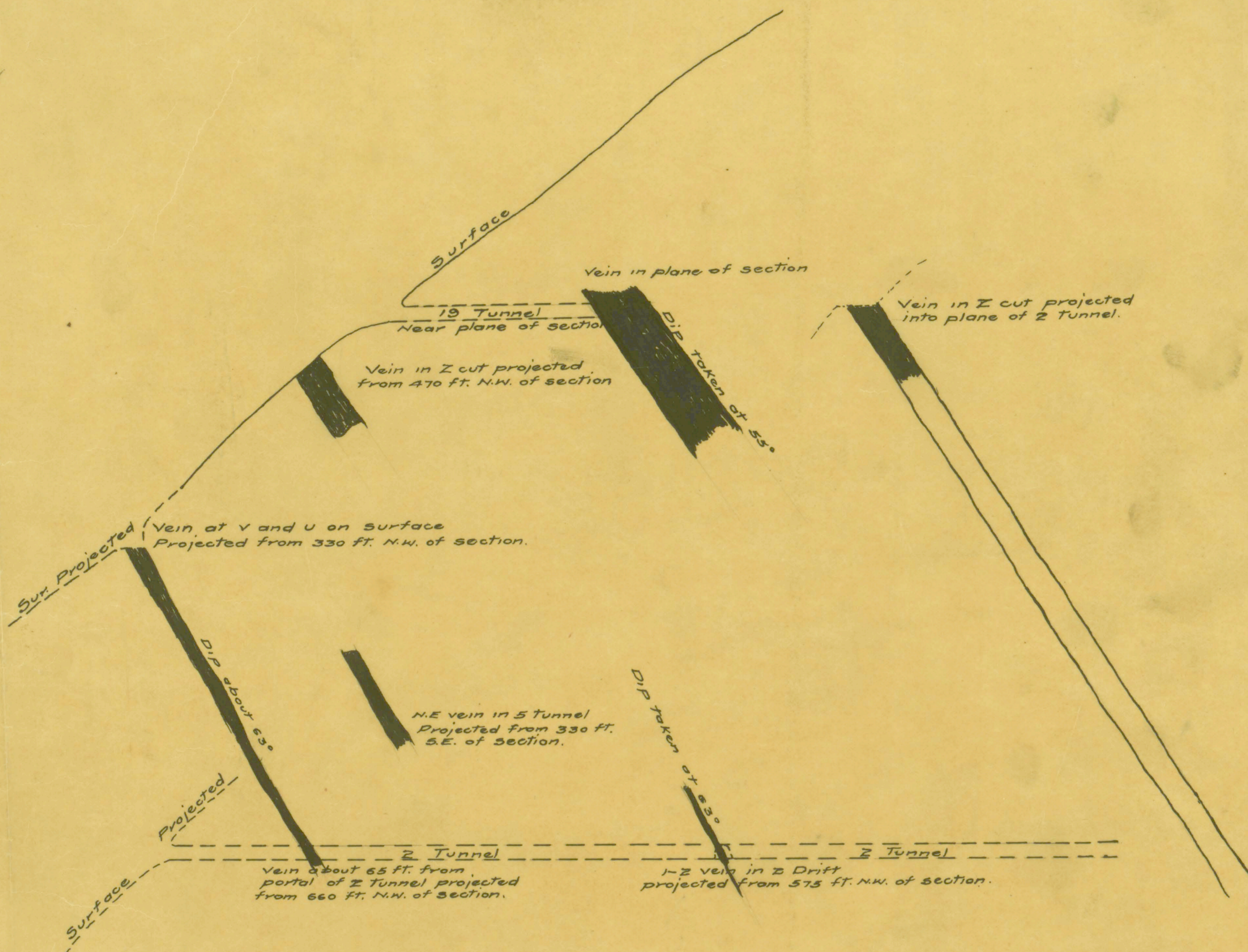
FIGURE 4 SECTION THROUGH B-B LOOKING SOUTHERST WITH VEINS PROJECTED AS INDICATED Scale 1 inch = 40 feet July 19-19
