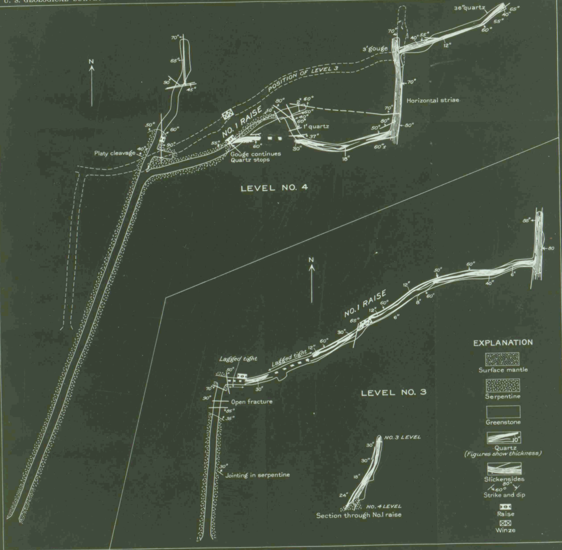
PLAN OF LEVELS 3 AND 4 AND SECTION THROUGH No. 1 RAISE ROBERT E. MINE, CURRY COUNTY, OREGON From Brunton compass survey by P. J. Shenon
