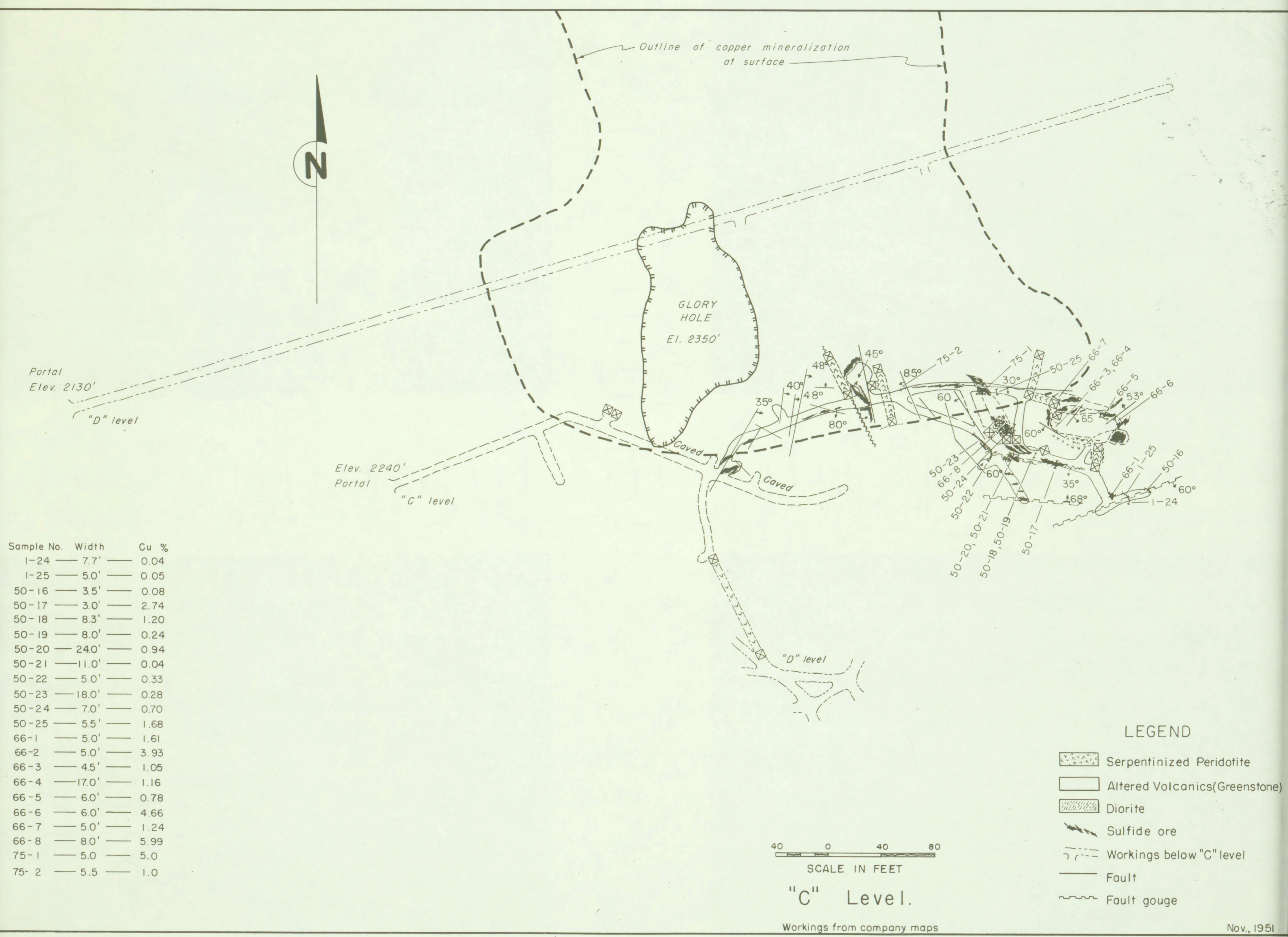
Figure 4. - Geologic and assay plan of Queen of Bronze mine, Takilma-Waldo district, Josephine County, Oregon.
