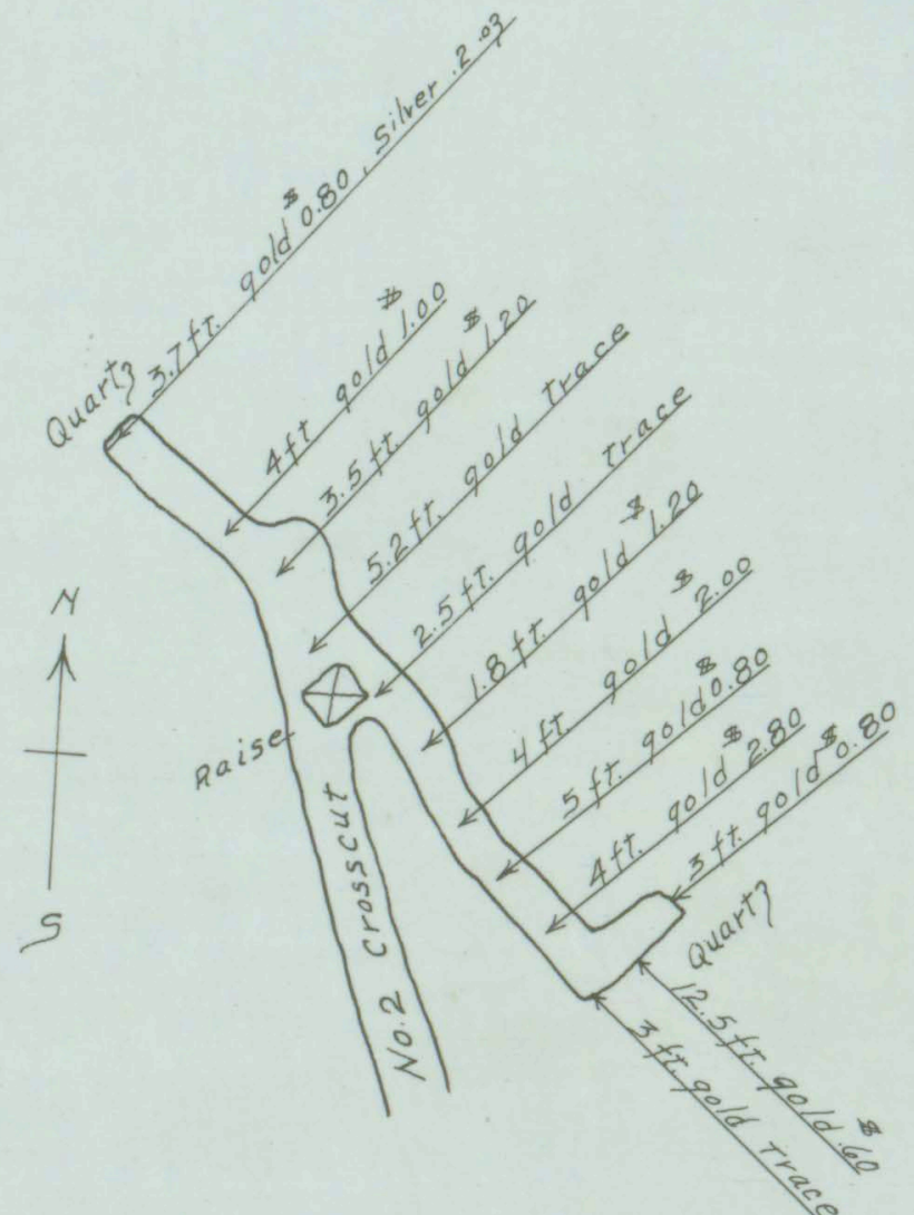
PLAN of No. 2 DRIFT Scale - 1 inch = 30 ft.
