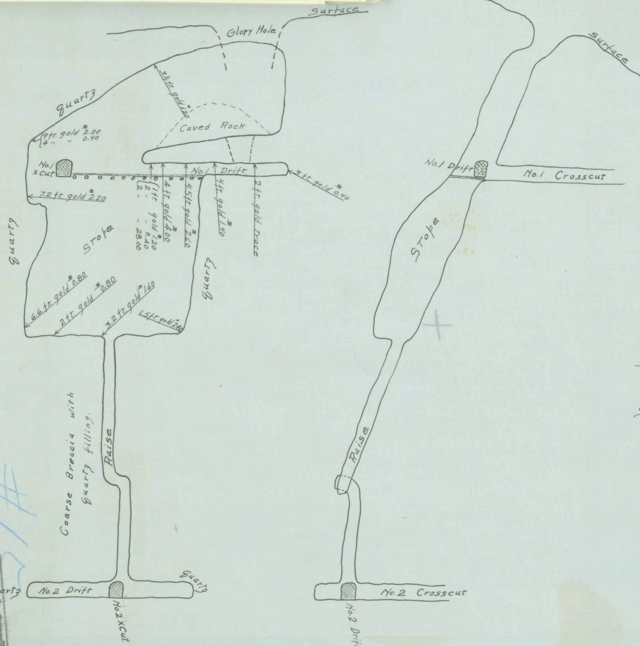
LONGITUDINAL STOPE SECTION Scale - 1 inch = 20 ft.
