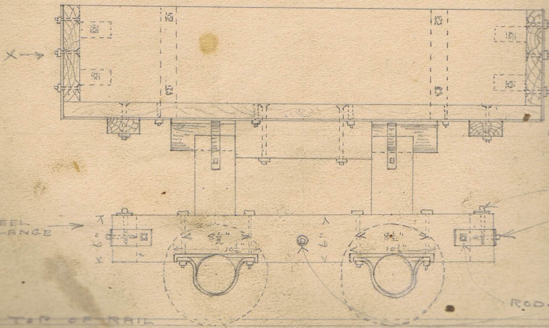
ELEVATION OF PUSH CAR
