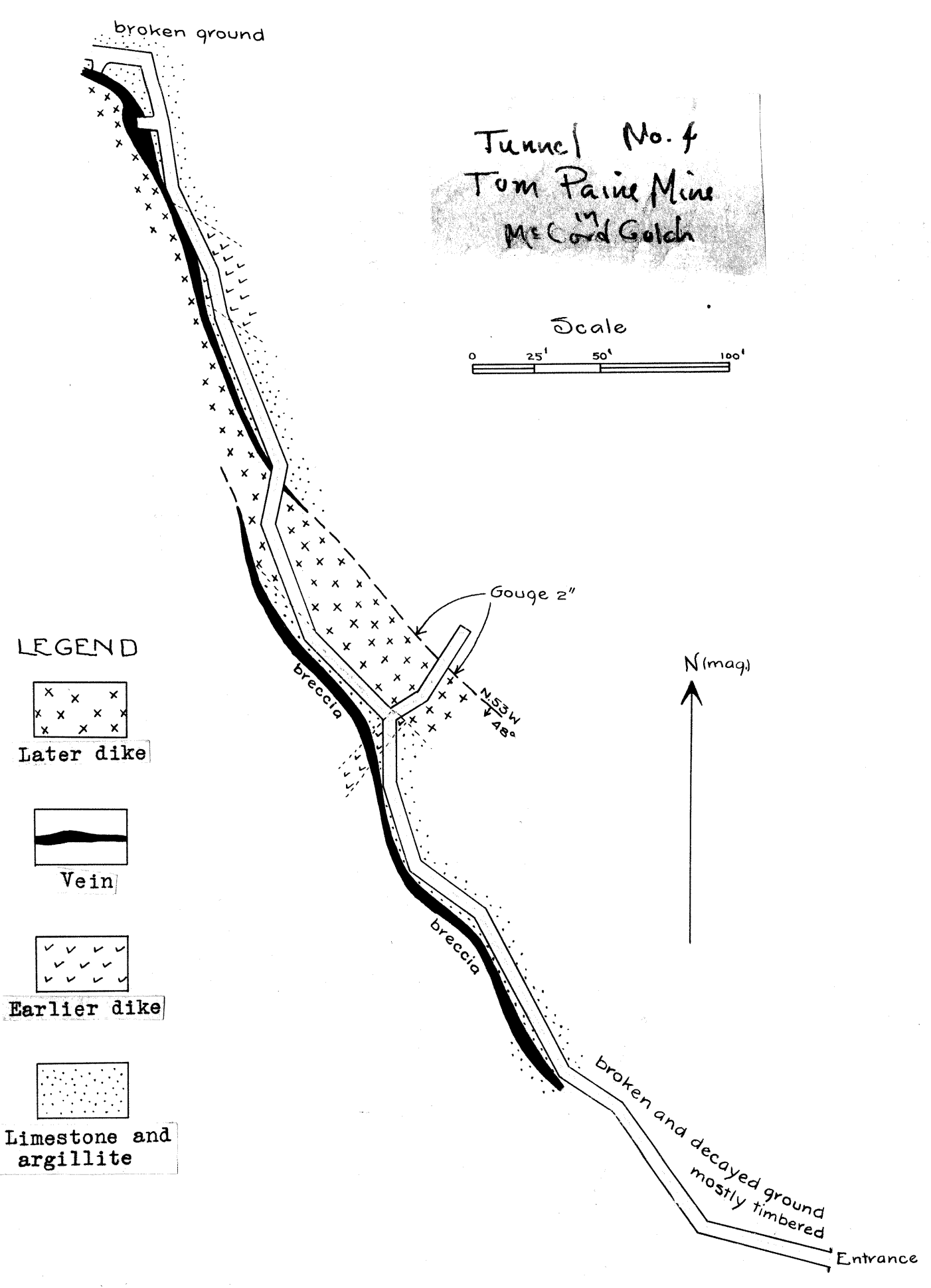
Reduce so this line is 4 inches long. Fig. 2 Tom Paine Mine in McCord Gulch
