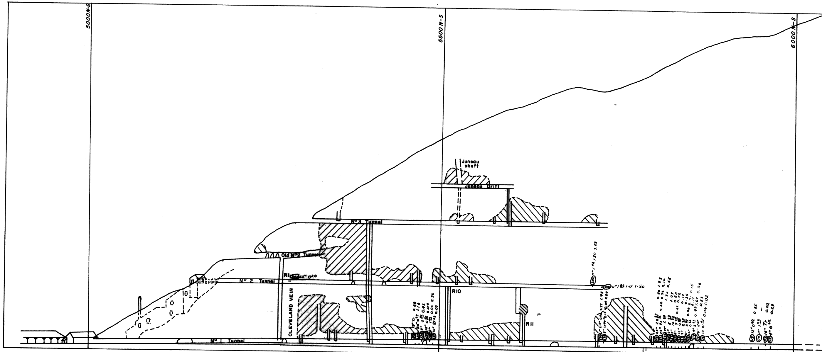
VERTICAL SECTION along STANDARD VEIN STANDARD MINE Grant County, Ore. 50 40 30 20 10 0 25 50 75 100 Direction of Section: N 76° E LEGEND Stopes on Main Standard Vein: /// Stopes on near by parallel veins: //
