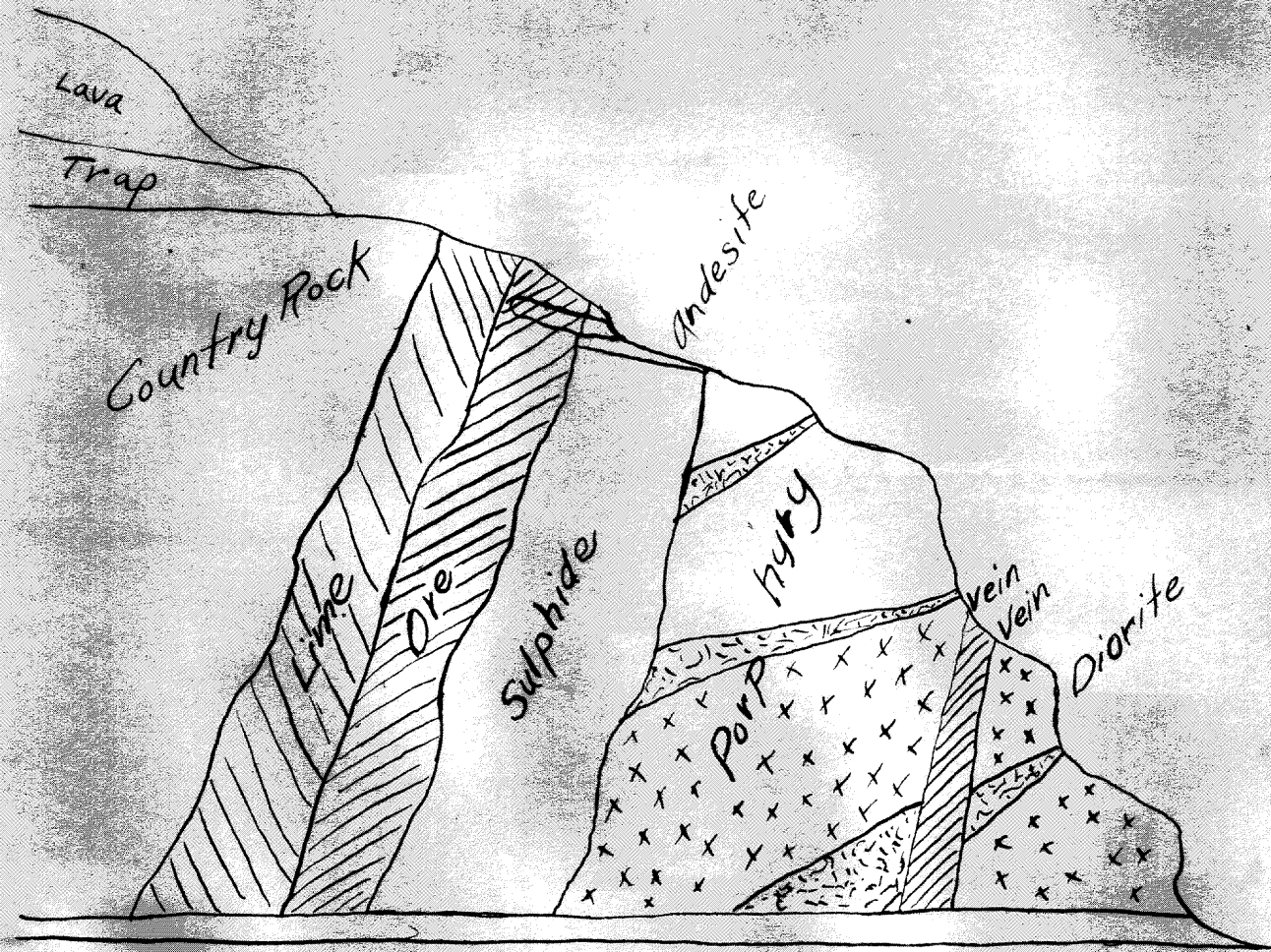
Gross section of Squaw Creek Mineral Belt
