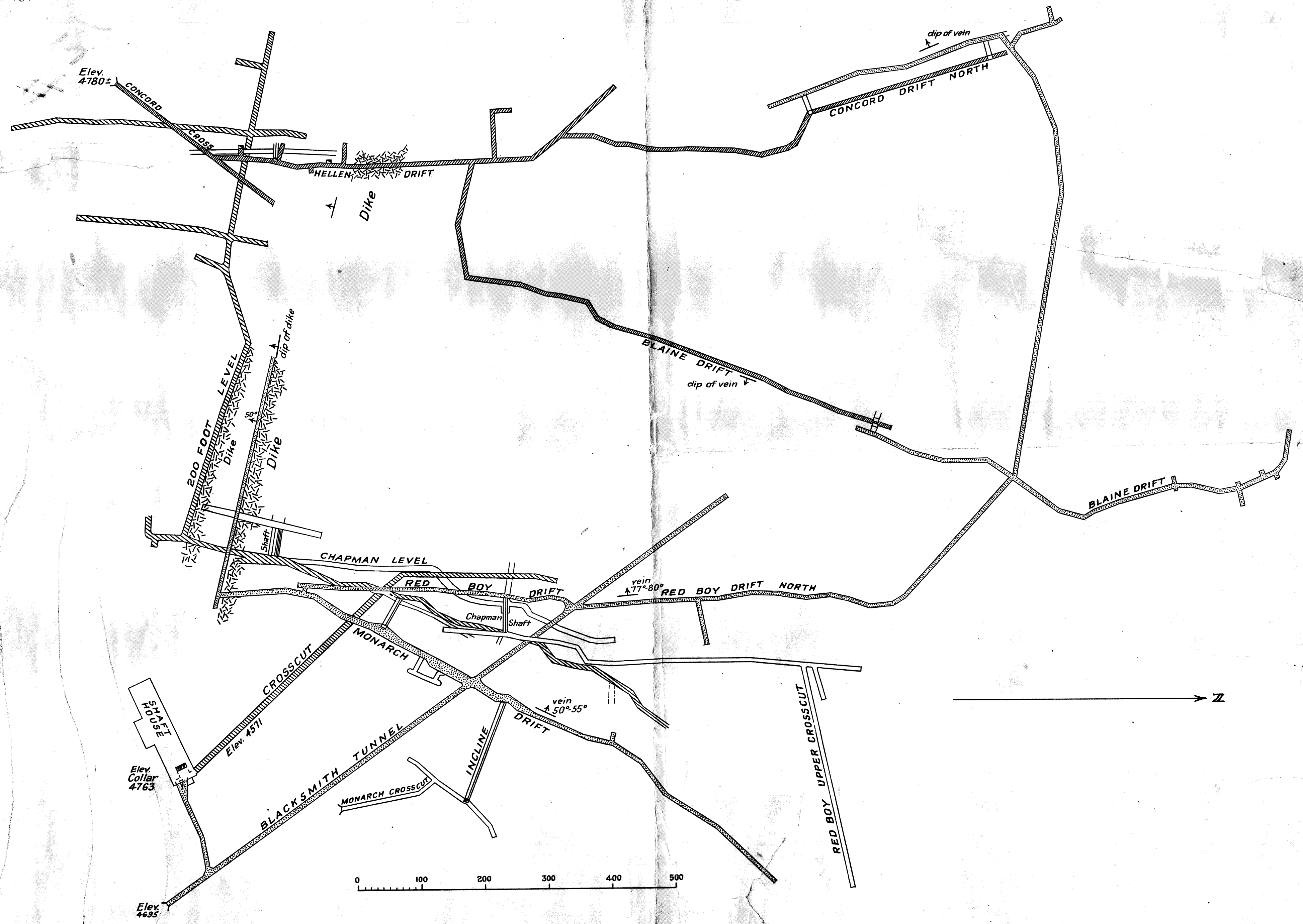
Fig. 29 Plan of Principal Workings of Red Boy Mine
