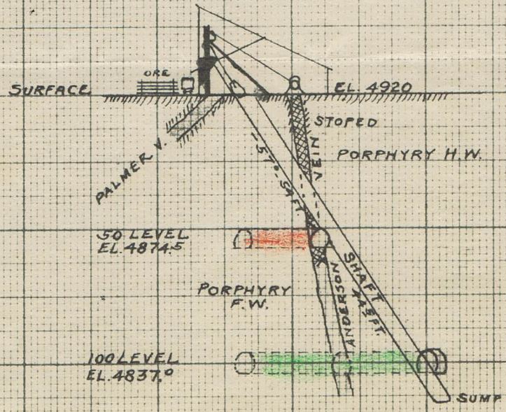
VERTICAL SECTION AT C OF SHAFT 1 INCH = 40 FEET A-B
