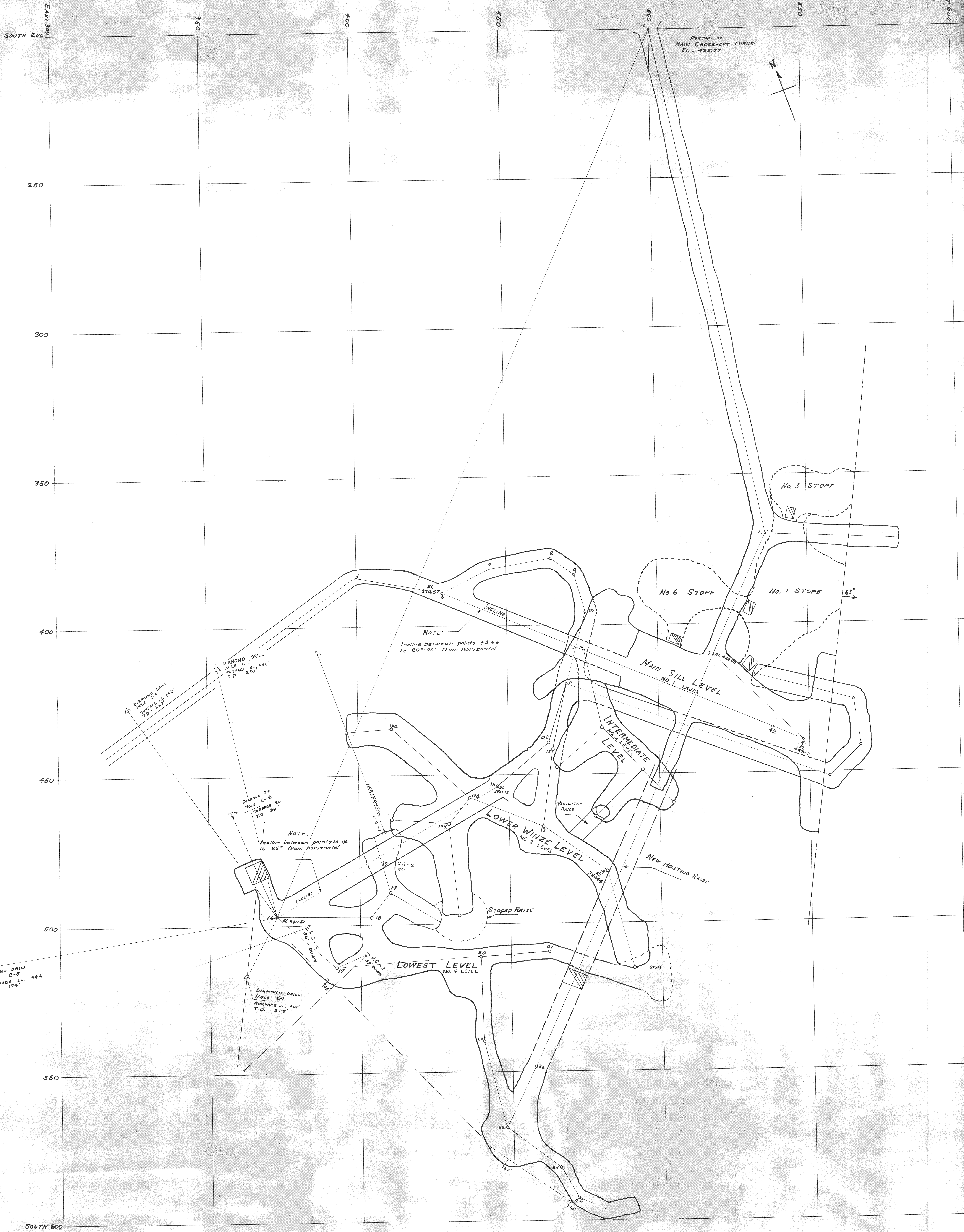
PLAN OF WORKINGS HORSE HEAVEN MERCURY MINE JEFFERSON COUNTY, OREGON SCALE: 1 IN. = 10 FT. DATE: APRIL 1936
