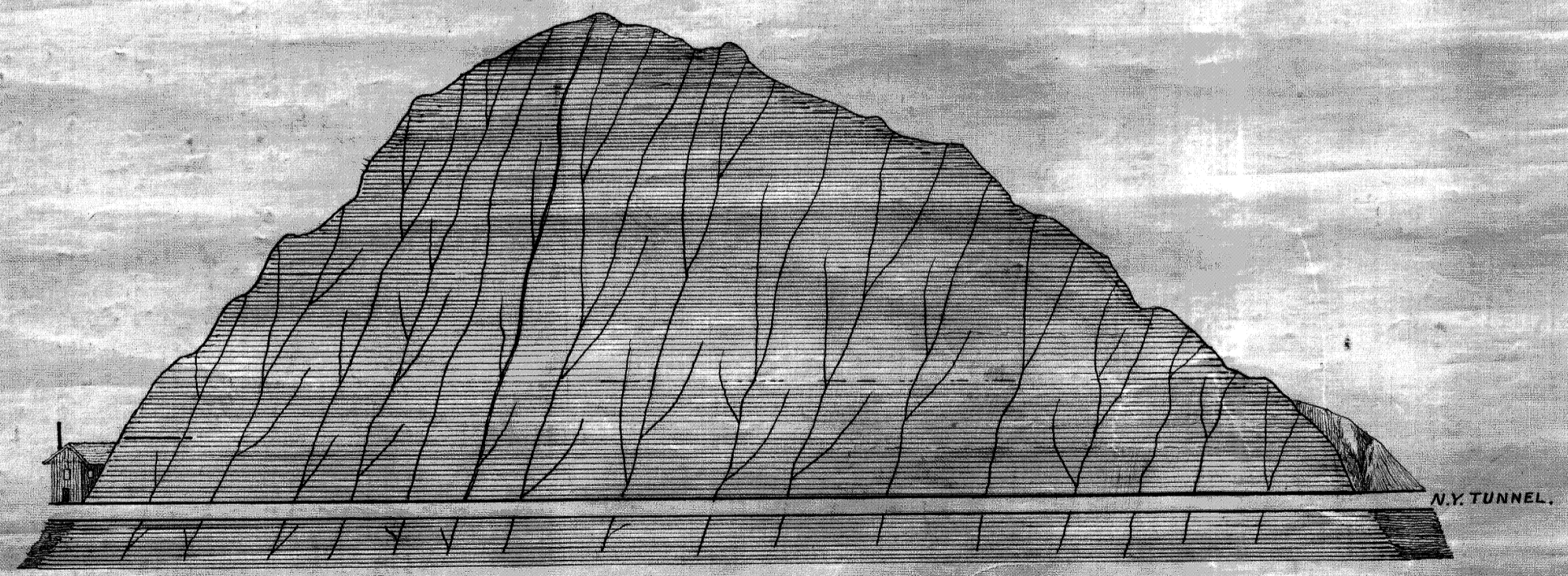
CROSS CUT THROUGH BALSLEY ELKHORN MOUNTAIN, on line of NEW YORK TUNNEL. Scale 1320 Feet to 1 Inch.
