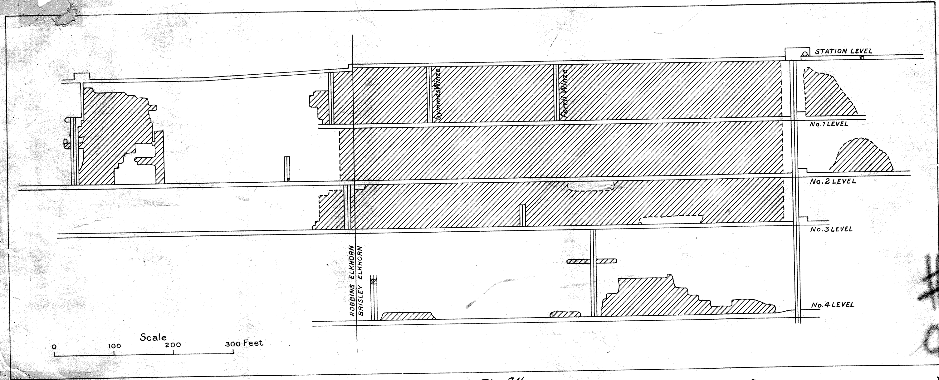
Fig. 24 Stepemap of Baisley-Elkhorn and Robbins-Elkhorn Mines Only stopes below tunnel level shown.
