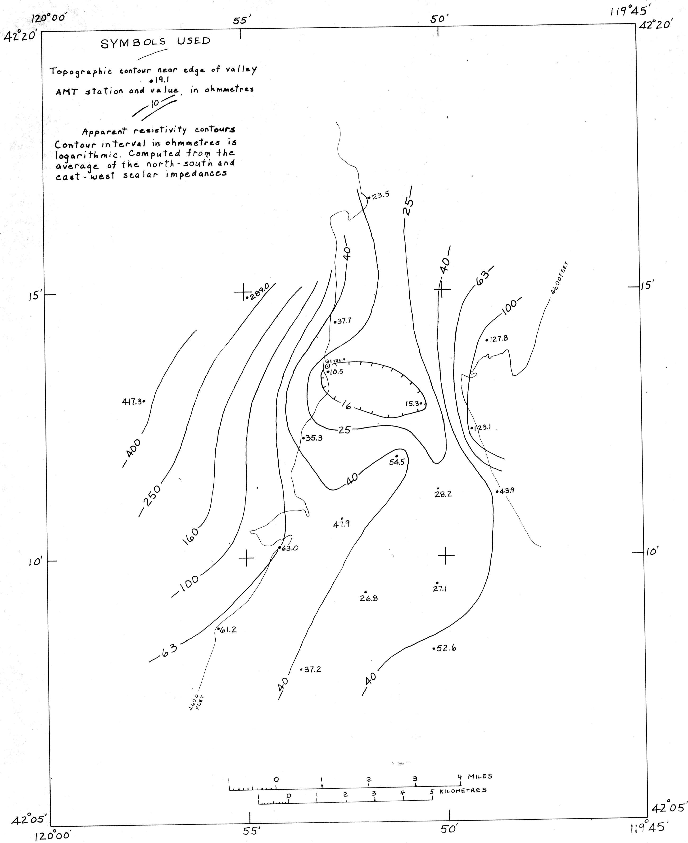
AUDIO-MAGNETOTELLURIC APPARENT RESISTIVITY MAPS SOUTHERN WARNER VALLEY, LAKE COUNTY, OREGON 285 HERTZ BY D. I. GREGORY AND R. J. MARTINEZ 1975
