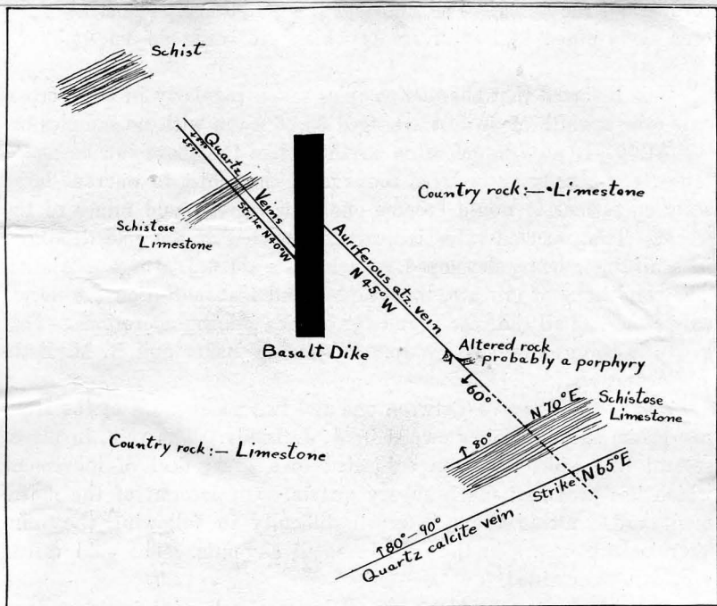
Fig. 93. Sketch showing Mullin veins.
