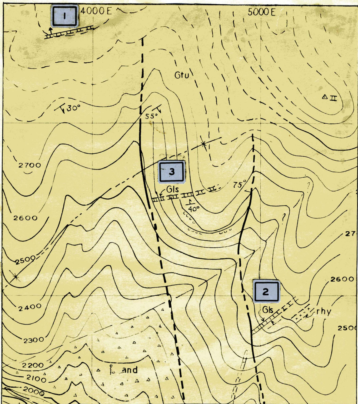
LOCATION OF LIMESTONE OCCURRENCES SAMPLED IN HOMESTEAD AREA BASE IS THE NORTHEAST CORNER OF DOGAMI MAP OF HOMESTEAD AREA BY J.E. ALLEN 1939 SCALE 1"=300'
