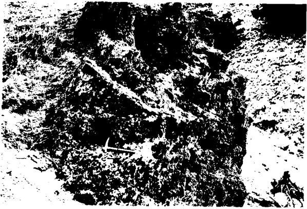
Outcrop siliceous "kidney" near upper end of claims. Shale replacement
