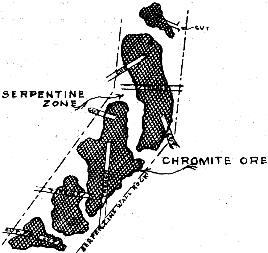
AJAX MINE ORE OCCURRENCE
