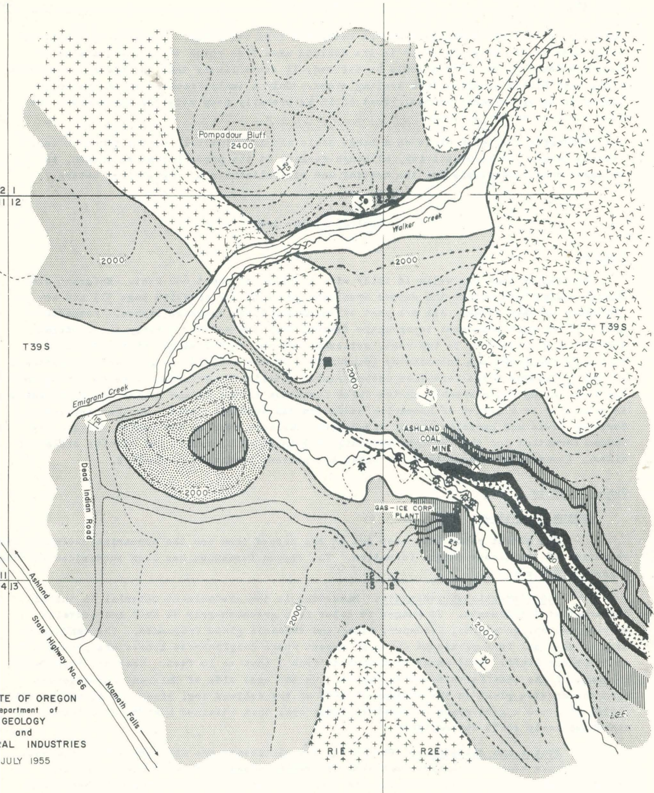
Geology of Area Around Gas-Ice Corp. Plant Near Ashland, Oregon.
