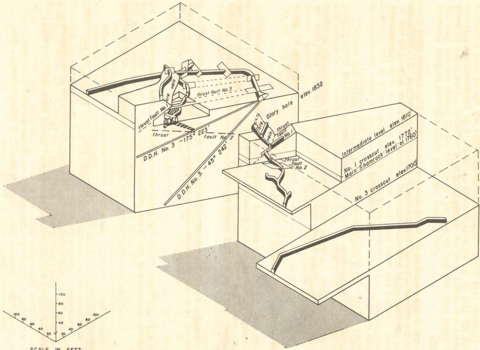
Figure 6. - Block diagram, Shamrock mine workings, Jackson County, Oreg.
