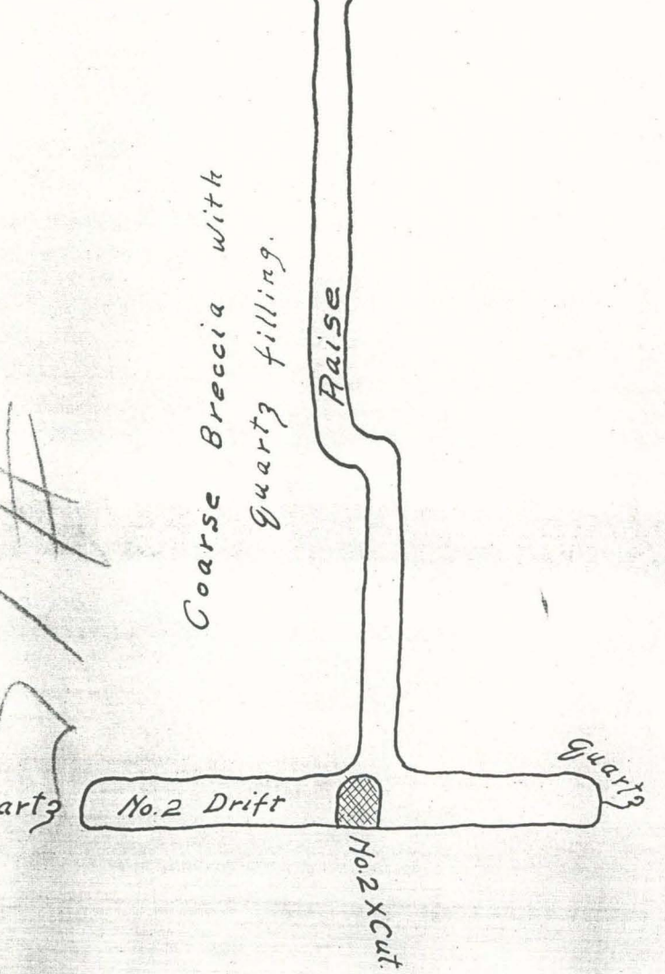
LONGITUDINAL STOPE SECTION Scale - 1 inch = 20 ft.
