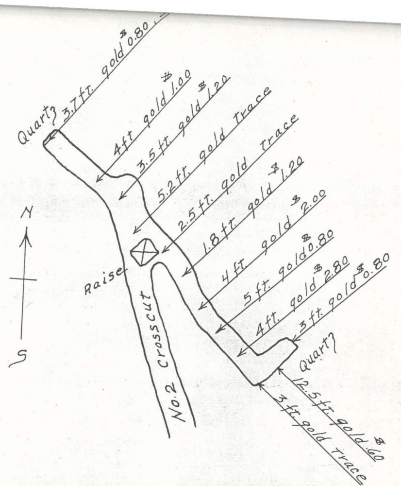
PLAN of No. 2 DRIFT Scale - 1 inch = 30 ft.
