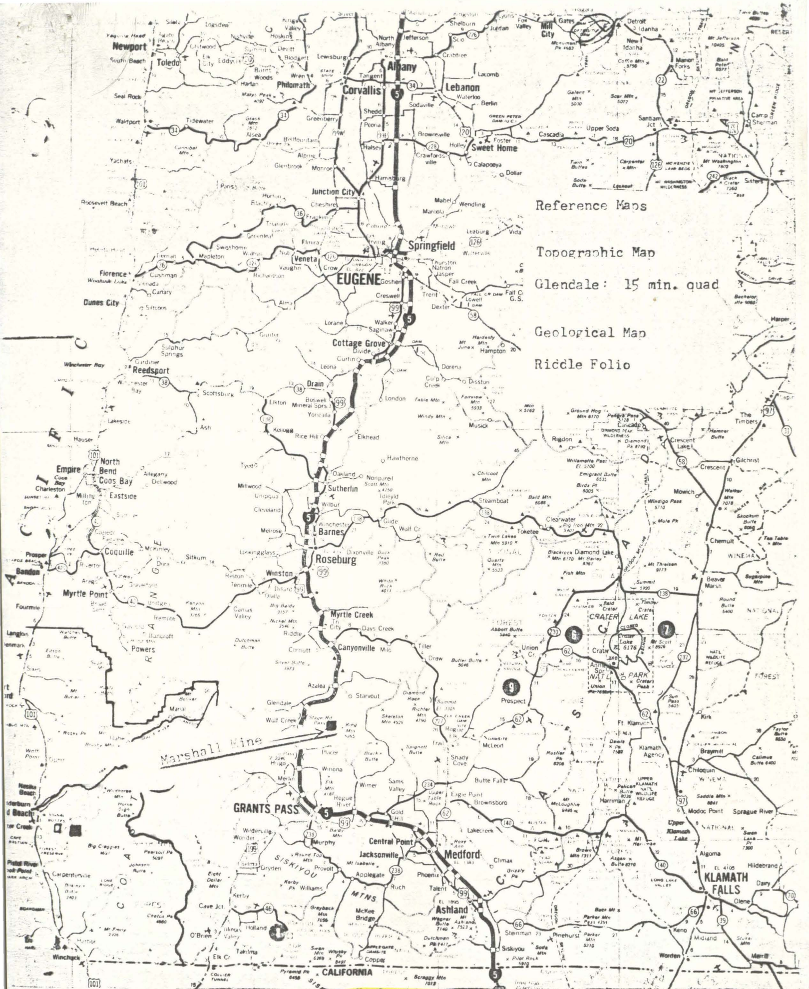
INDEX MAP OF THE MARSHALL (DOROTHEA) MINE JOSEPHINE COUNTY, OREGON
