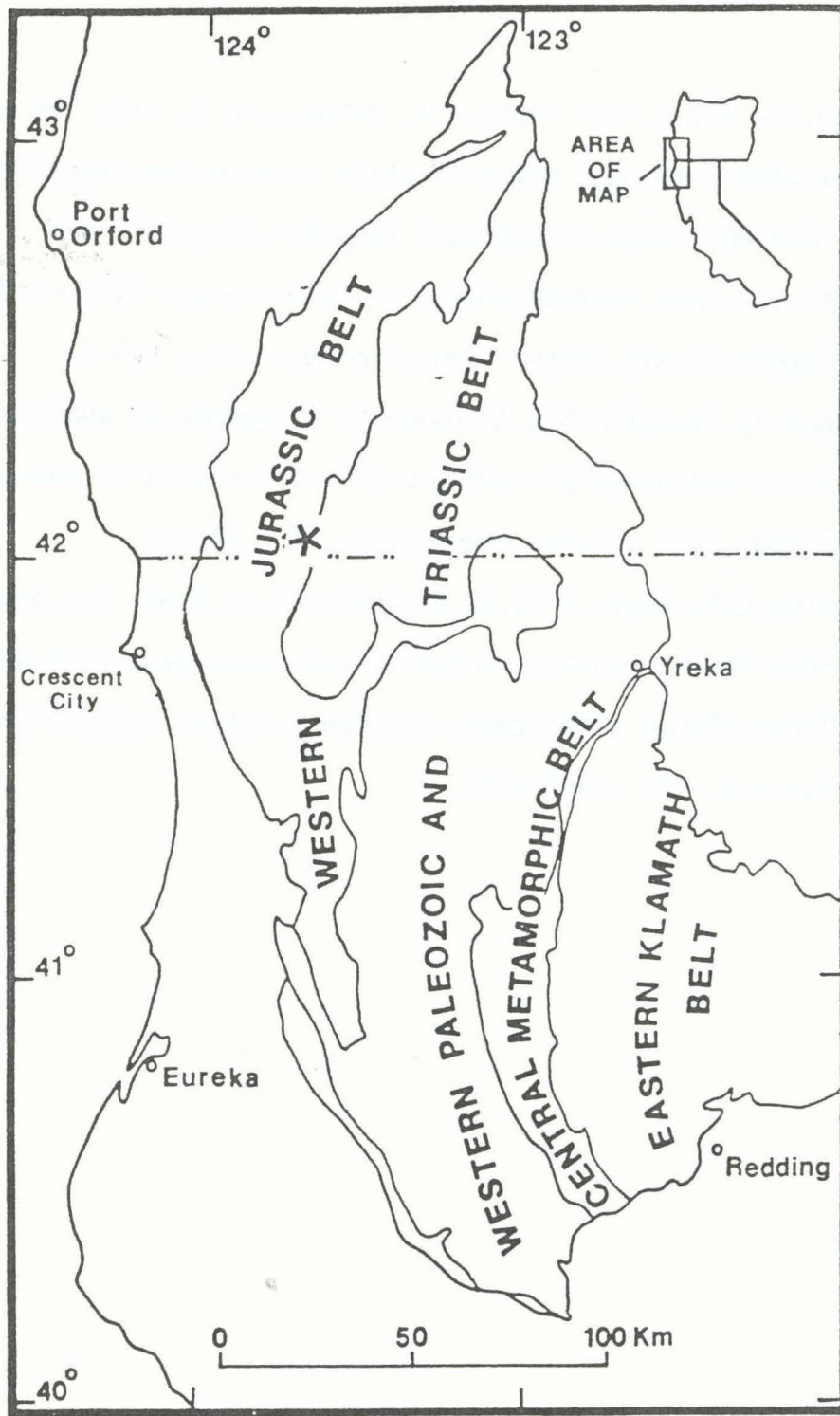
Figure 1. Index map showing lithotectonic belts of the Klamath Mountains, Oregon and California. Star shows location of the Turner-Albright sulfide deposit.
