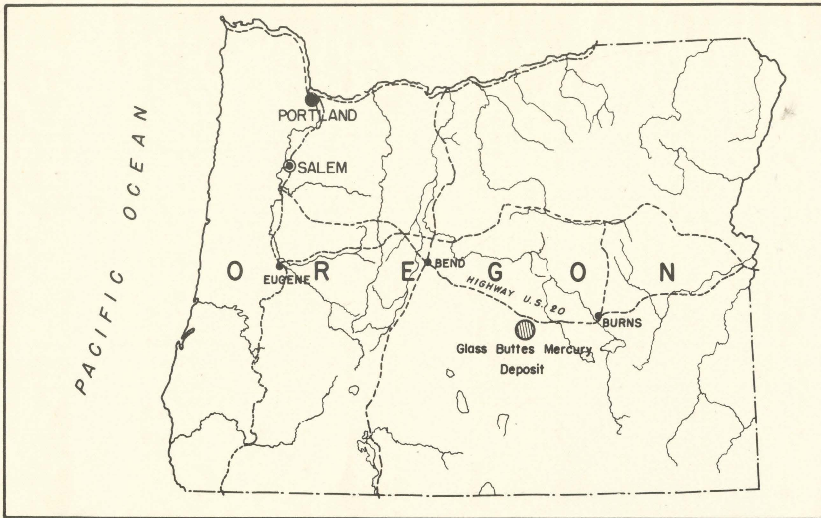
Fig. 1, Index Map of Oregon Showing Location of Glass Buttes Deposit
