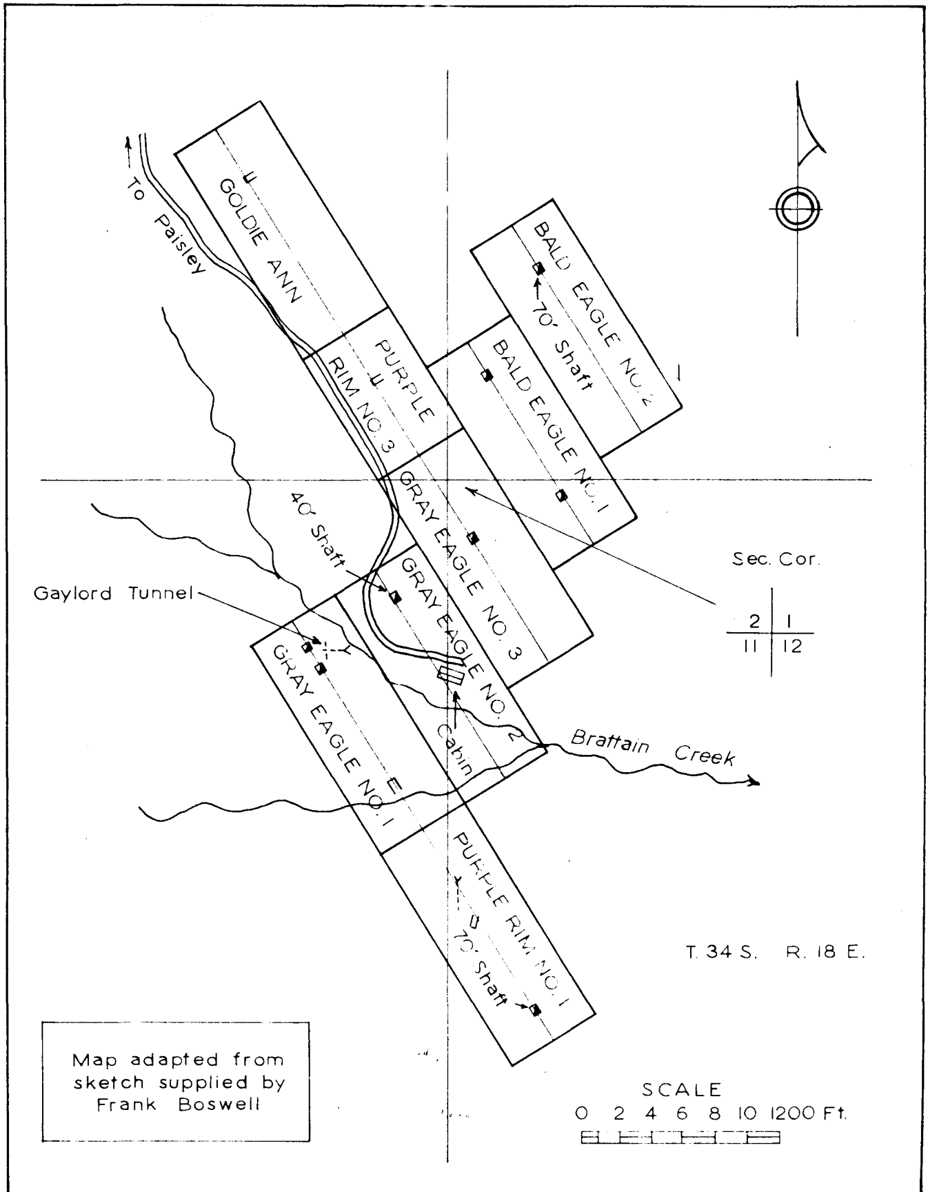
Claim map of lead-zinc deposit near Paisley, Lake County, Oregon.
