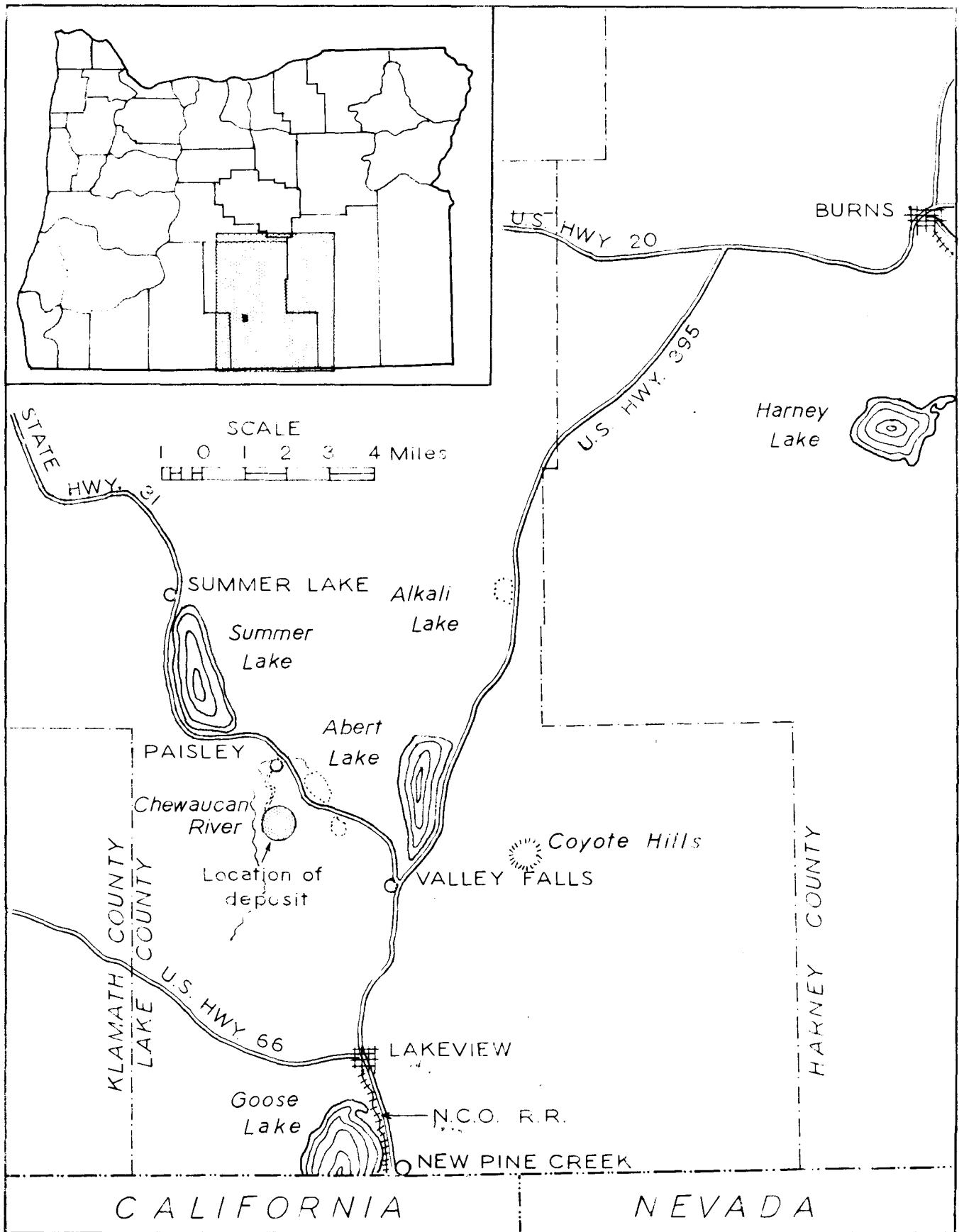
Index map showing location of lead-zinc deposit near Paisley, Lake County, Oregon.
