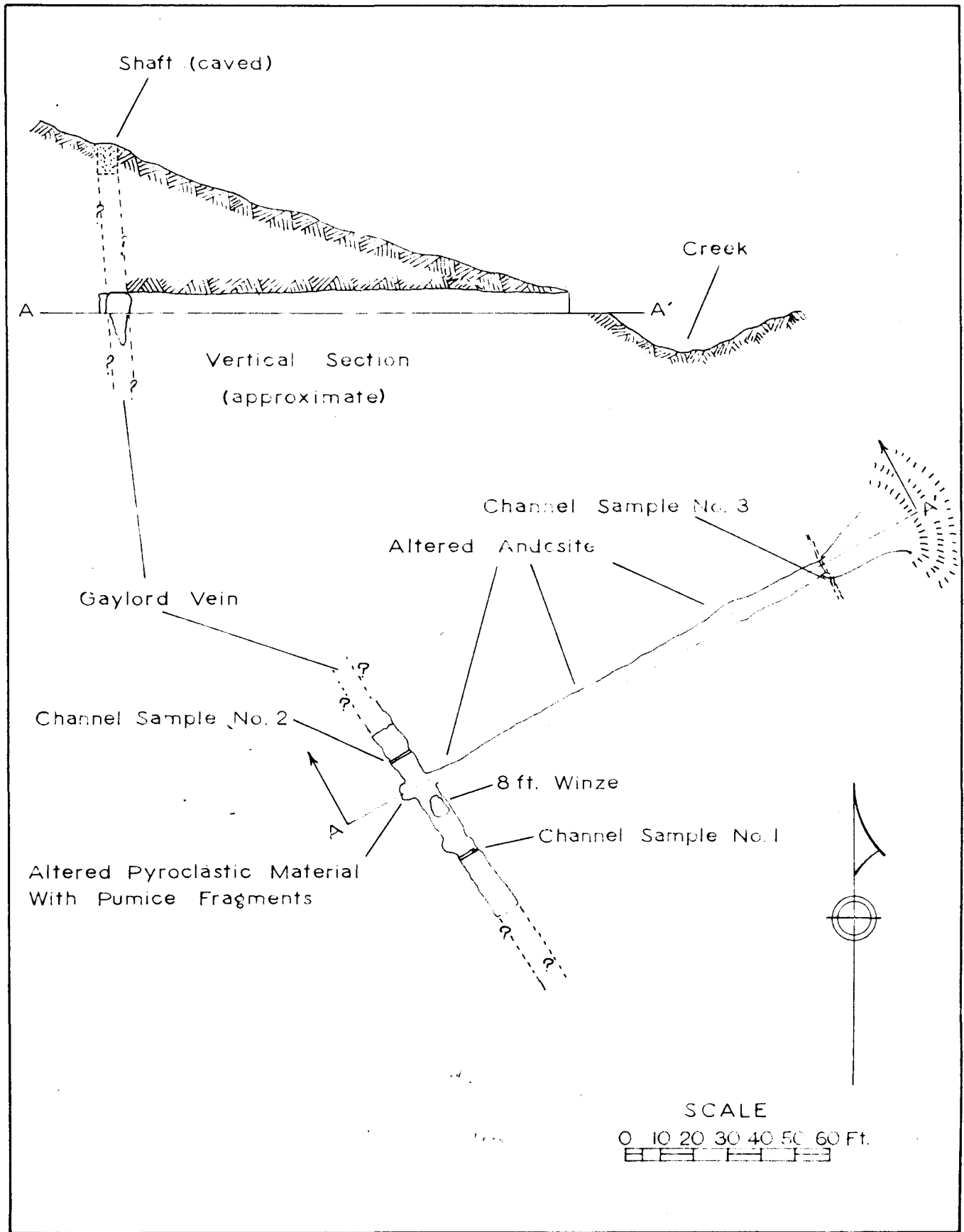
Sketch map of Gaylord tunnel and vein, Lake County, Oregon.
