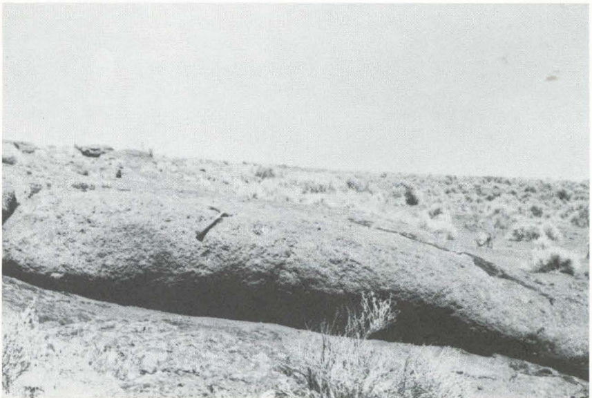
Figure 7. Another view of a thin flow unit of pahoehoe lava on Dudeck Ridge. Extremes in temperature acting on coarse-grained, open-textured basalt produce granular disintegration.
