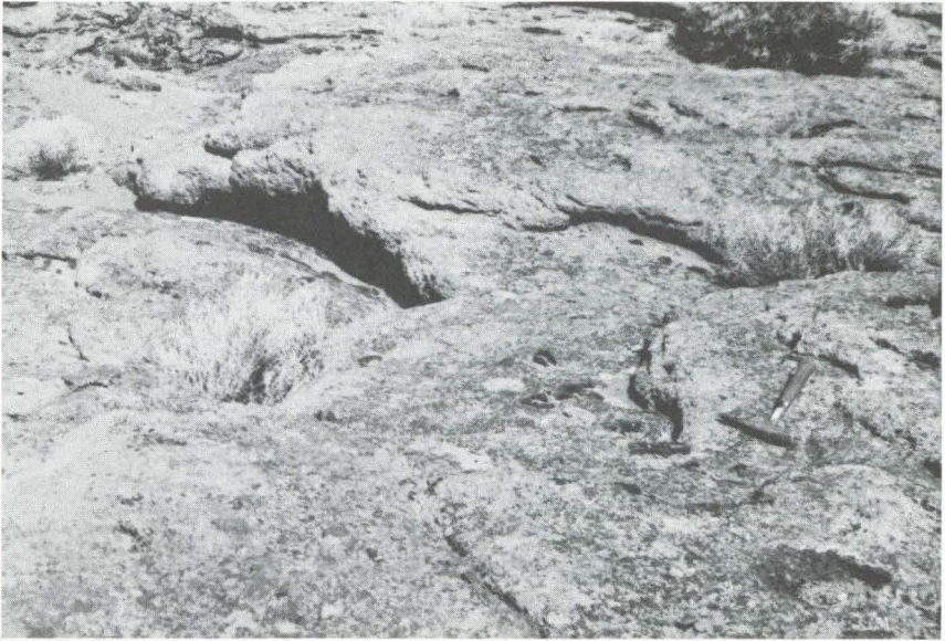
Figure 6. Exposure of weathered pahoehoe lava on Dudeck Ridge showing hummocky bulbous flow units of the sunstone-bearing basalt. Fine-grained weathering products are blown away and the coarser fragments accumulate in depressions.
