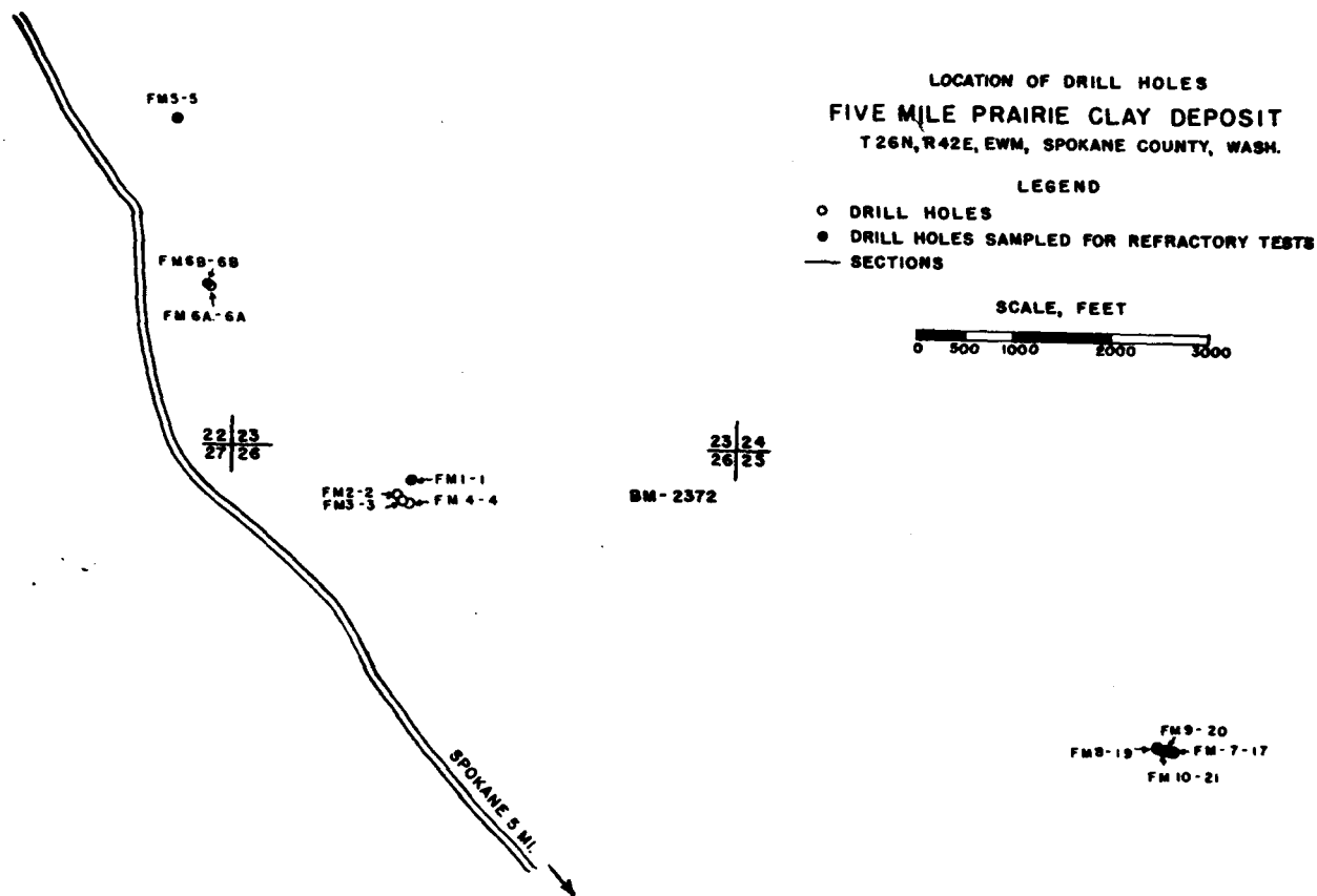
Figure 33. - Map showing the location of drill holes for the Five-Mile Prairie clay deposit, Spokane County, Wash., and holes selected for ceramic tests.
