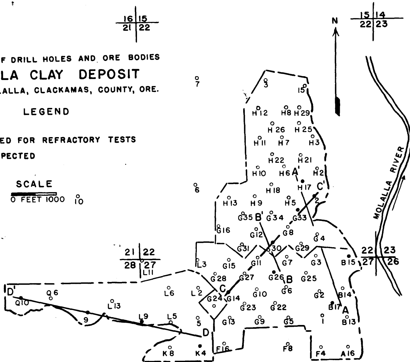
Figure 13. - Map showing location of drill holes for the Molalla clay deposit, Clackamas County, Oreg., and the holes selected for ceramic tests.
