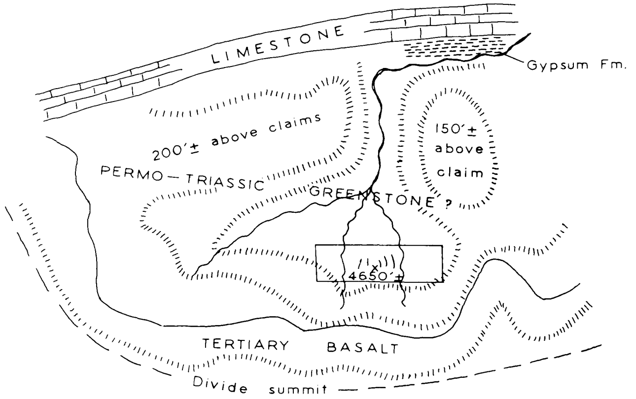
Generalized sketch map of magnetiferous area
