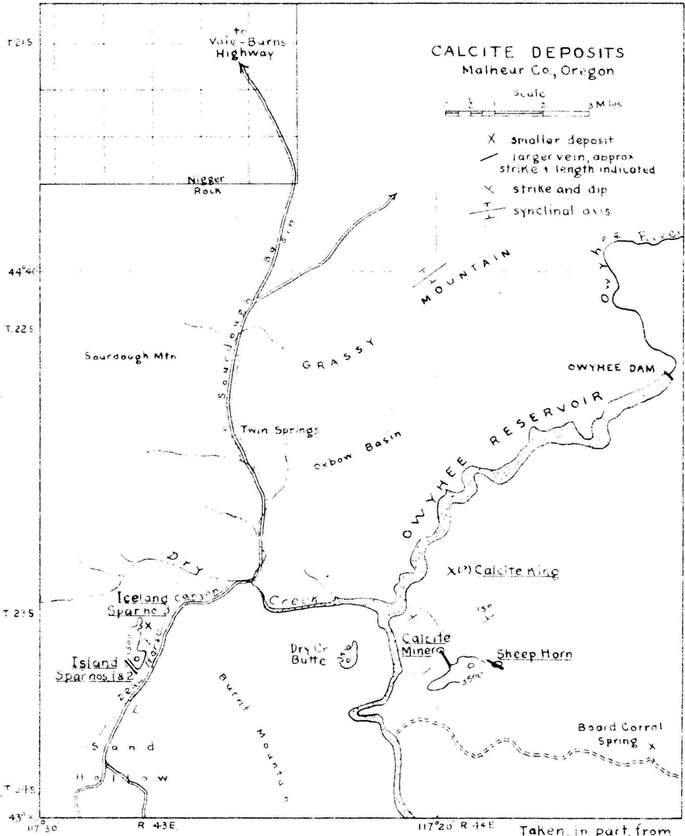
Figure 2. Location of Calcite Deposits, Malheur Co., Oregon
