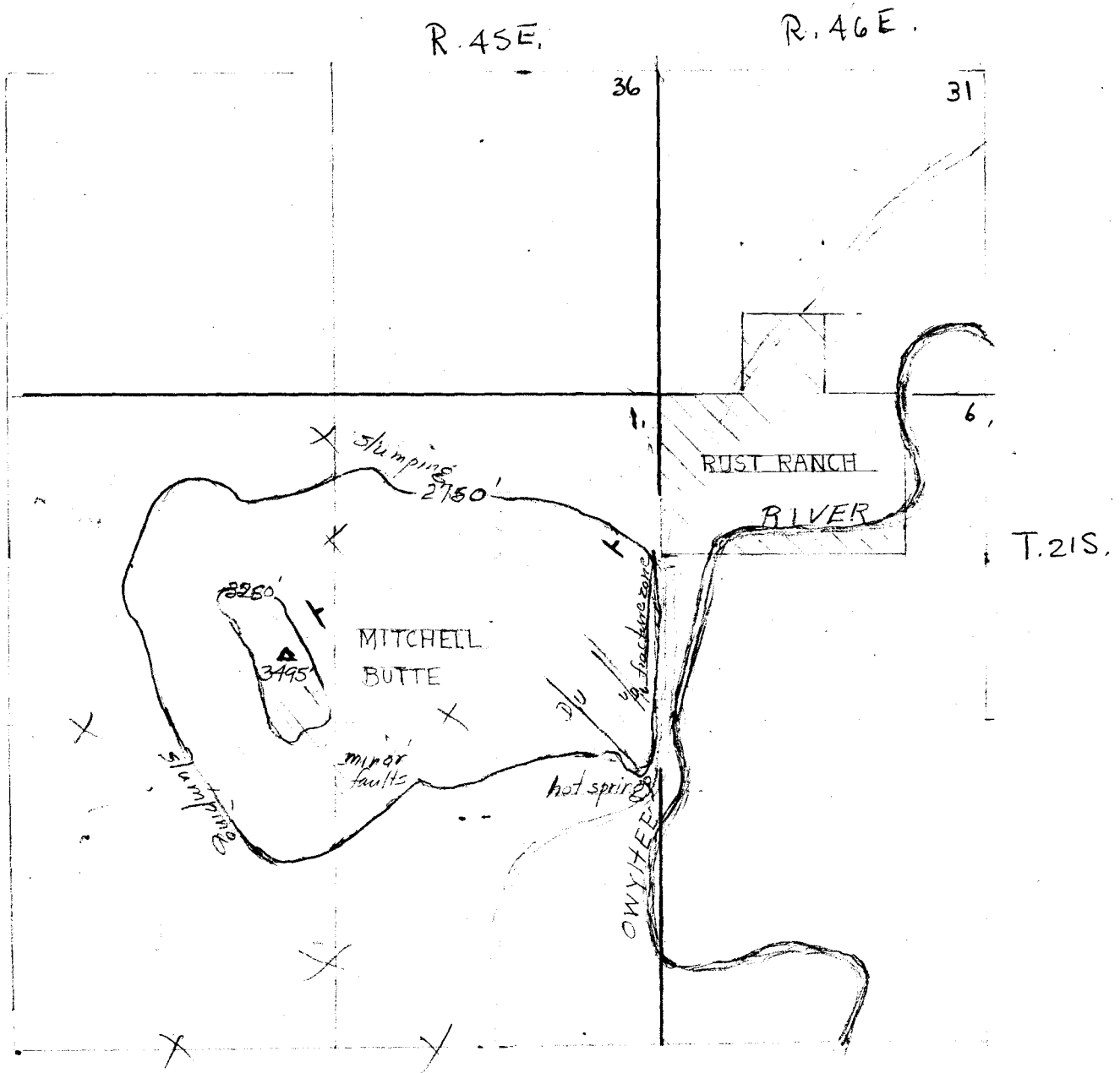
Figure 1. SKETCH MAP OF STRUCTURES SHOWN BY MITCHELL BUTTE
