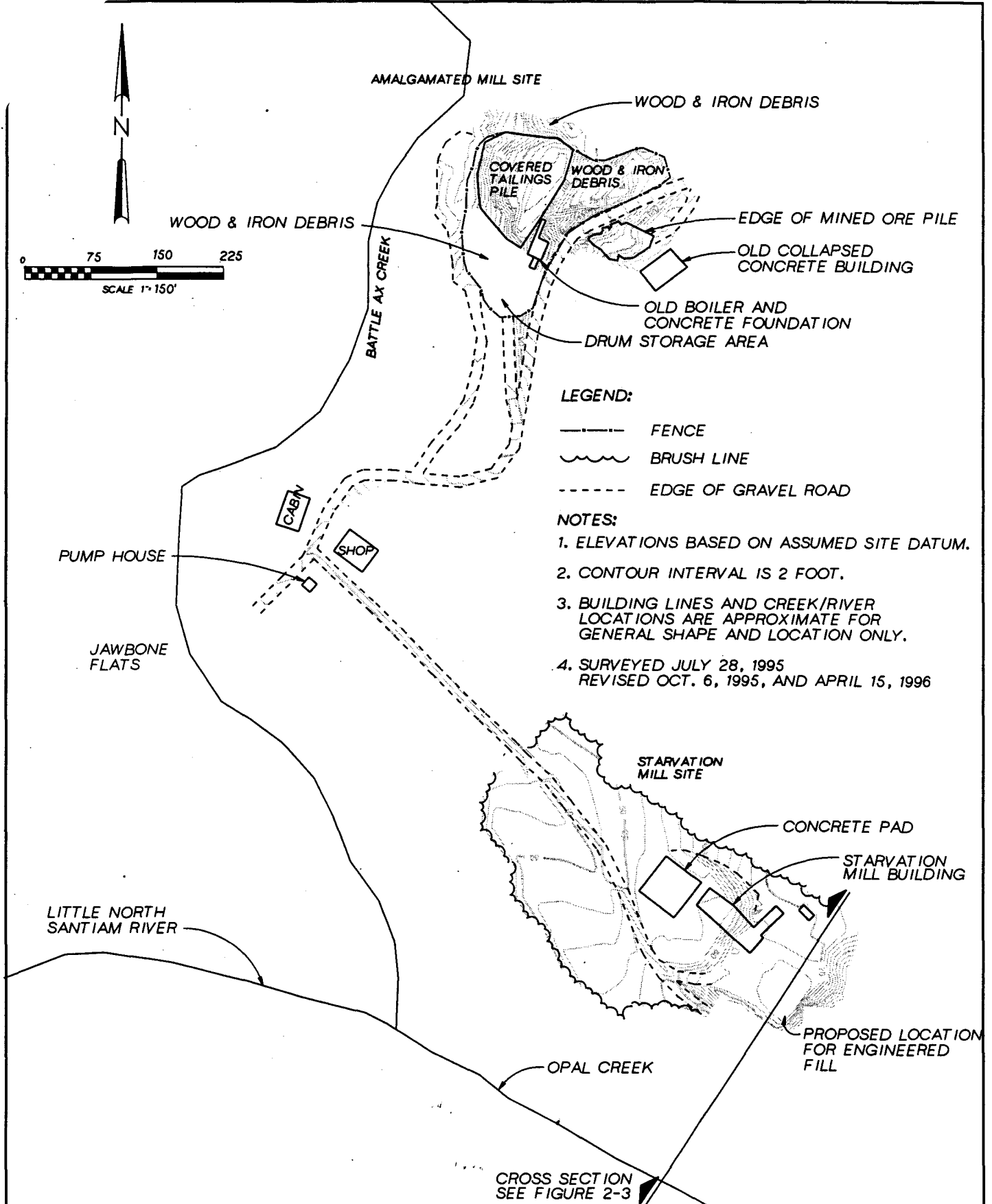
FIGURE 2-2 SITE MAP AMALGAMATED MILL FEASIBILITY STUDY
